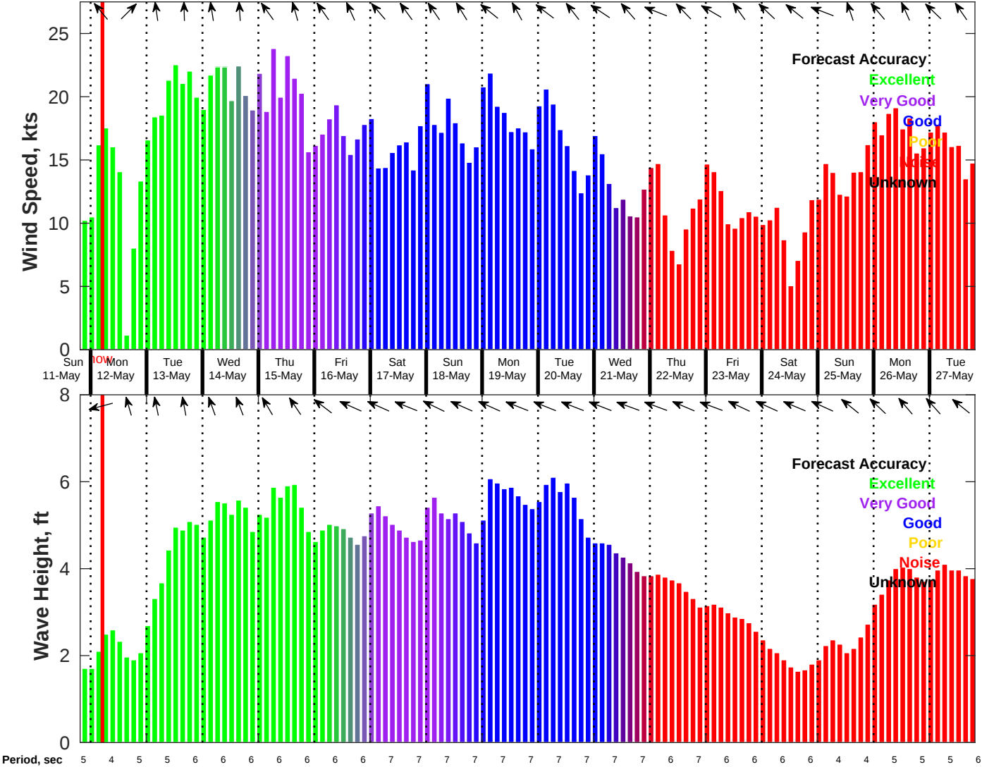
Wind & Wave Forecast for Tampnet P2378 South Texas Cable Route Geophysical from 11-May-2025 20:00:00 to 27-May-2025 20:00:00
