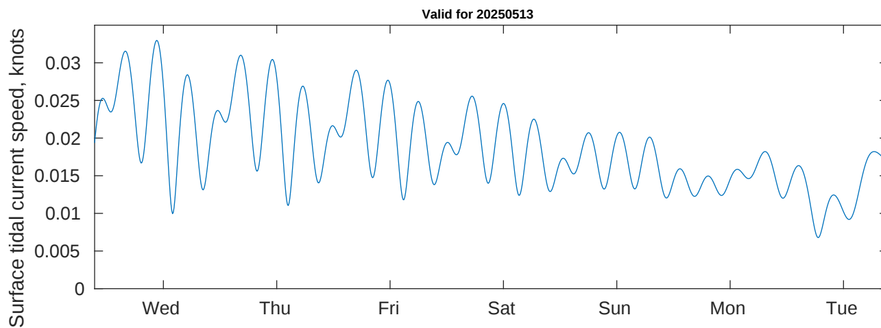
Tidal Currents and Heights for Benthic Solutions South Africa HF Site1 at 20250513
