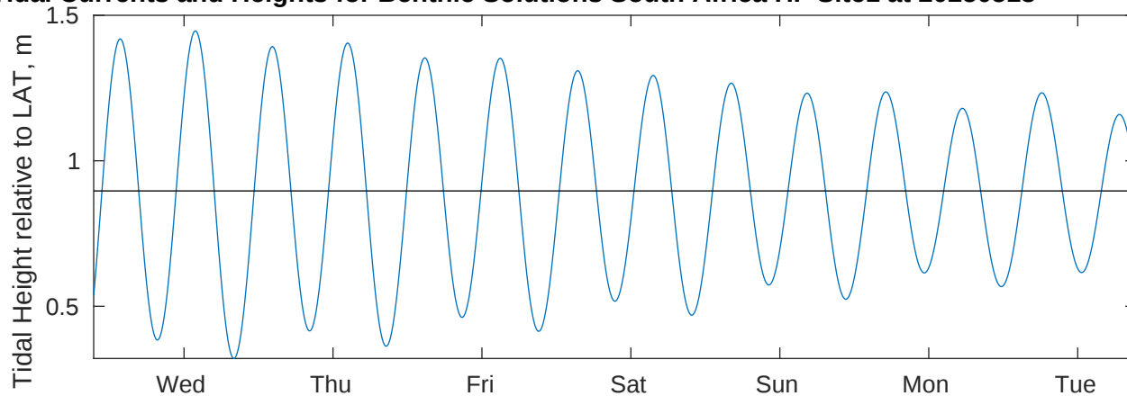
Tidal Currents and Heights for Benthic Solutions South Africa HF Site1 at 20250513
