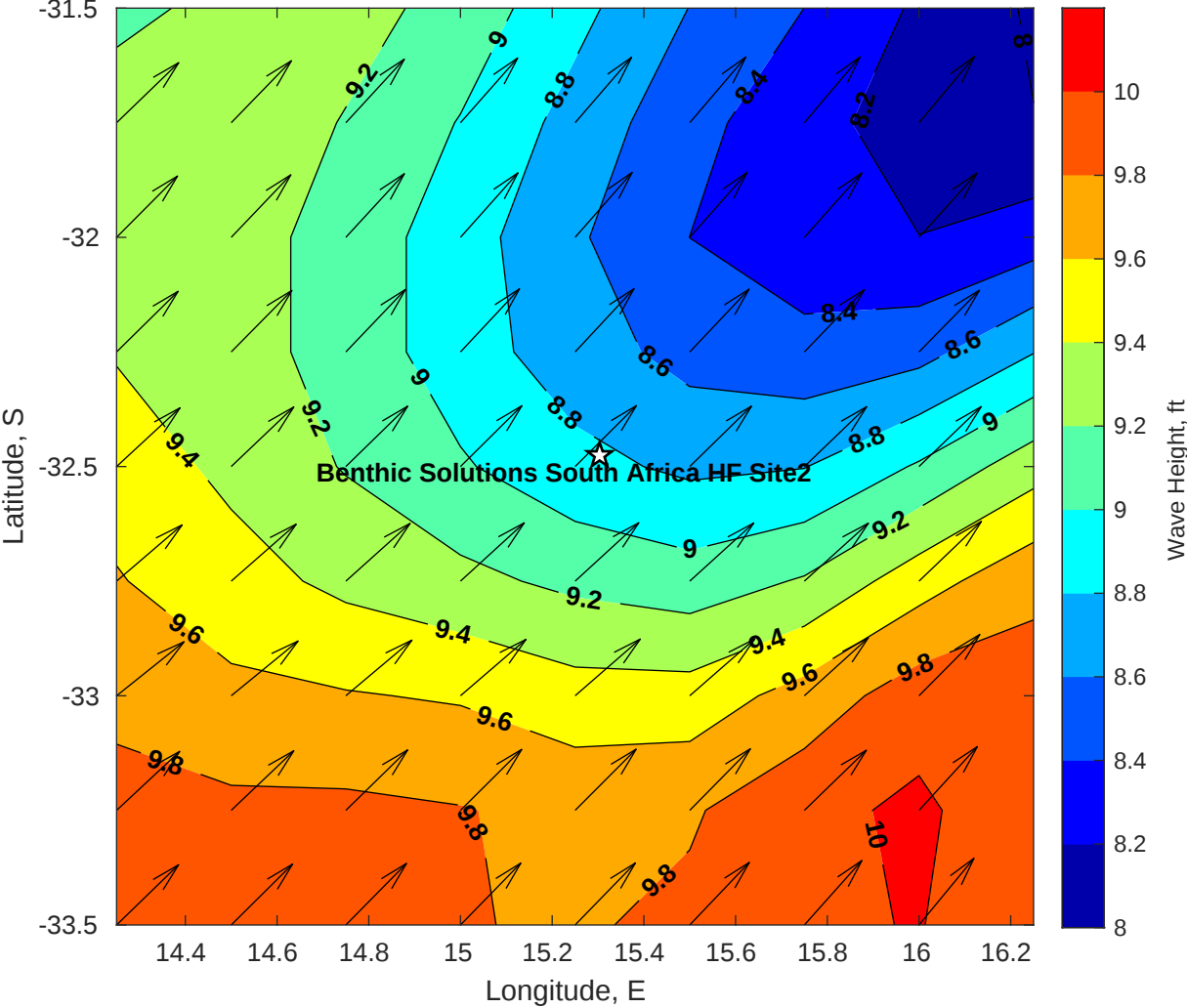
Wave Height (ft) for Benthic Solutions South Africa HF Site2 at 13-May-2025 09:00:00
