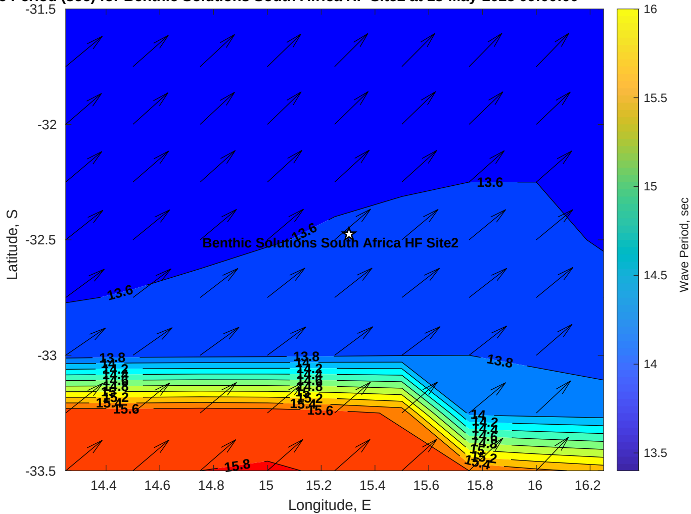
Wave Period (sec) for Benthic Solutions South Africa HF Site2 at 13-May-2025 09:00:00
