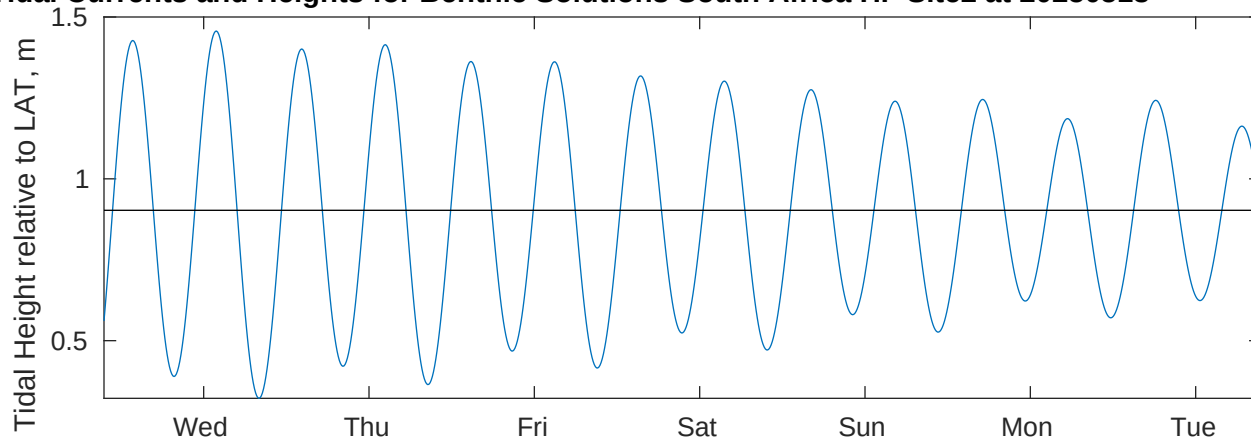
Tidal Currents and Heights for Benthic Solutions South Africa HF Site2 at 20250513
