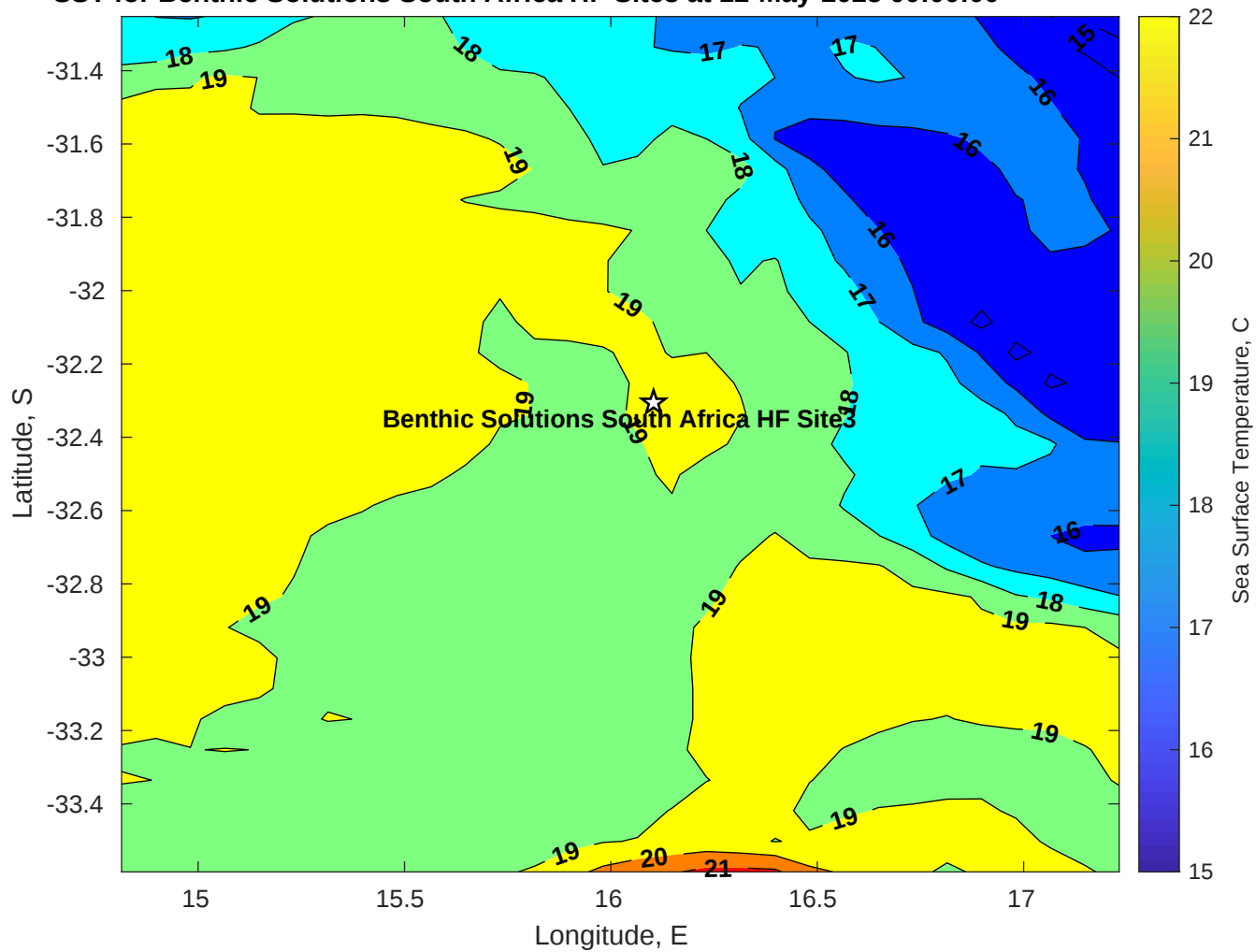
SST for Benthic Solutions South Africa HF Site3 at 12-May-2025 00:00:00
