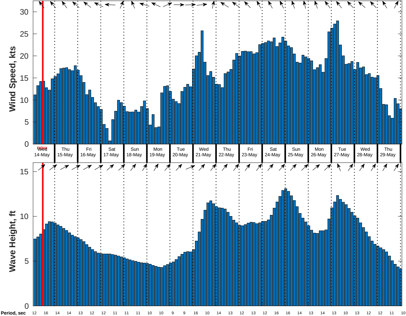
Wind & Wave Forecast for Benthic Solutions South Africa HF Site3 from 13-May-2025 02:00:00 to 29-May-2025 02:00:00
