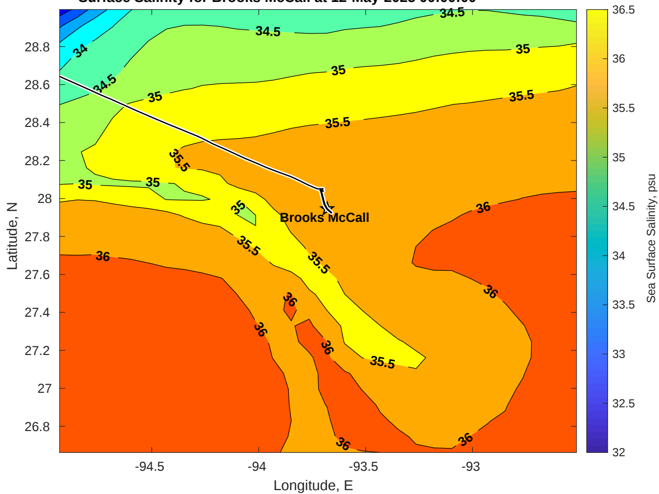
Surface Salinity for Brooks McCall at 12-May-2025 00:00:00
