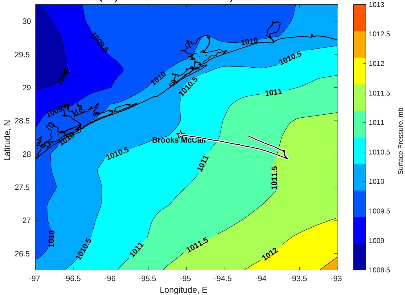
Surface Pressure (mb) for Brooks McCall at 13-May-2025 00:00:00
