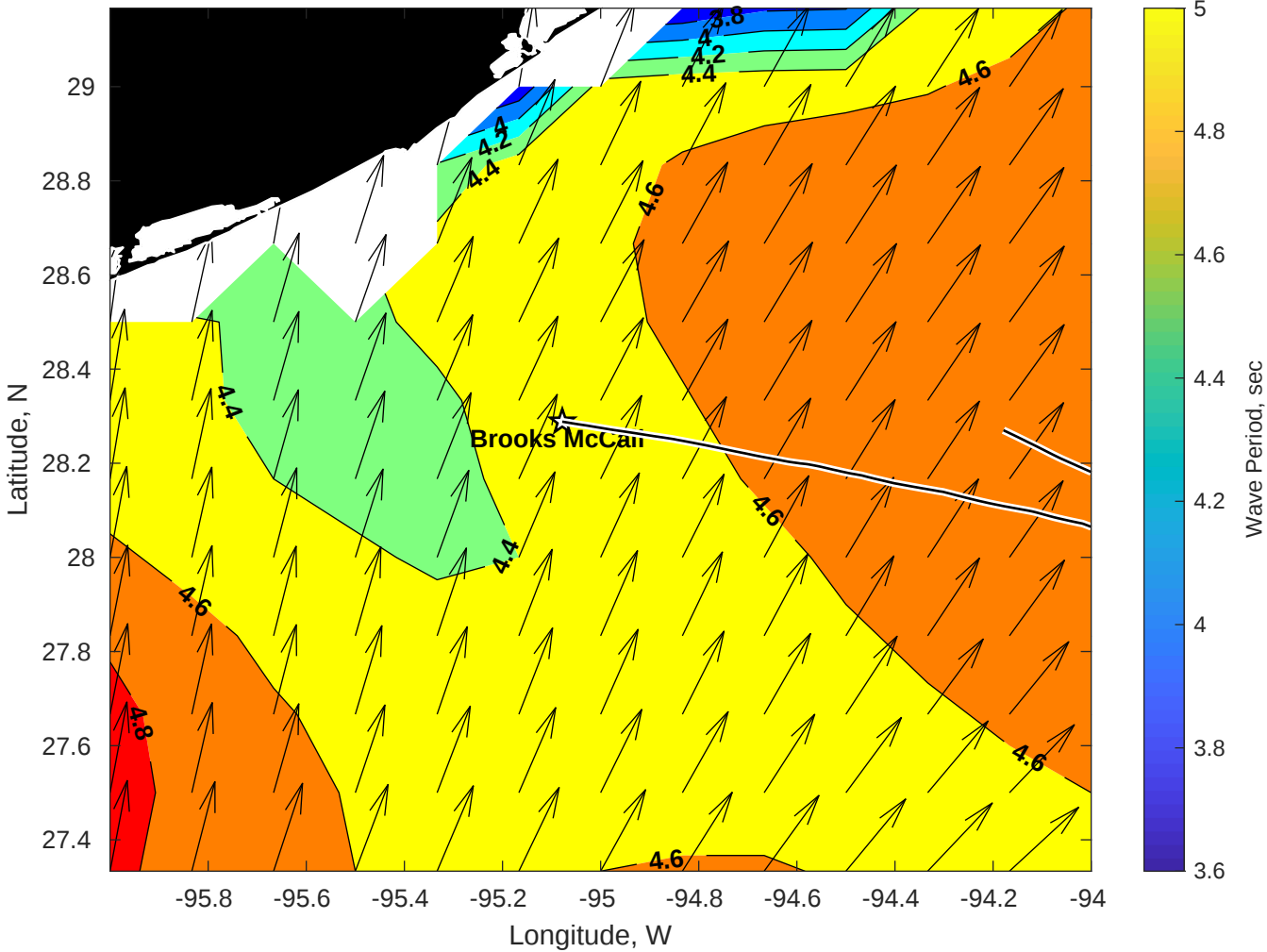
Wave Period (sec) for Brooks McCall at 13-May-2025 09:00:00
