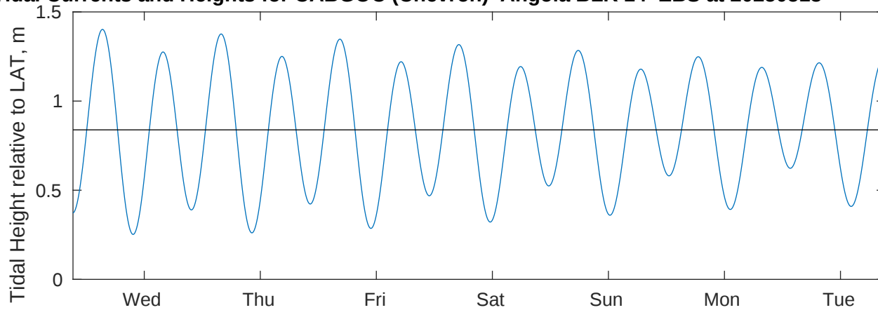
Tidal Currents and Heights for CABGOC (Chevron) Angola BLK 14 EBS at 20250513
