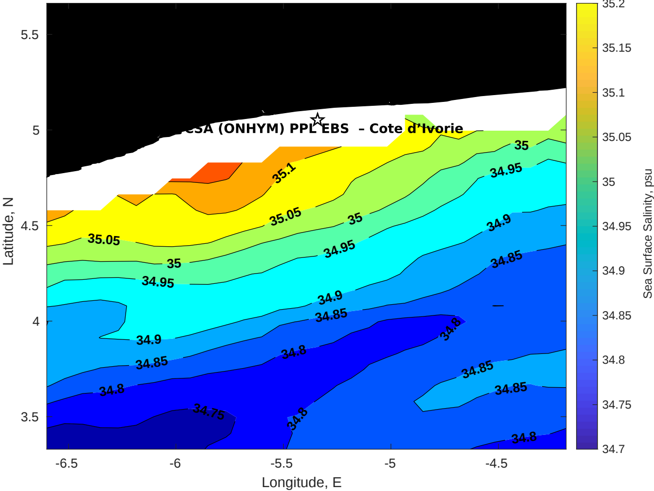
Surface Salinity for CSA (ONHYM) PPL EBS - Cote d'Ivoire at 12-May-2025 00:00:00
