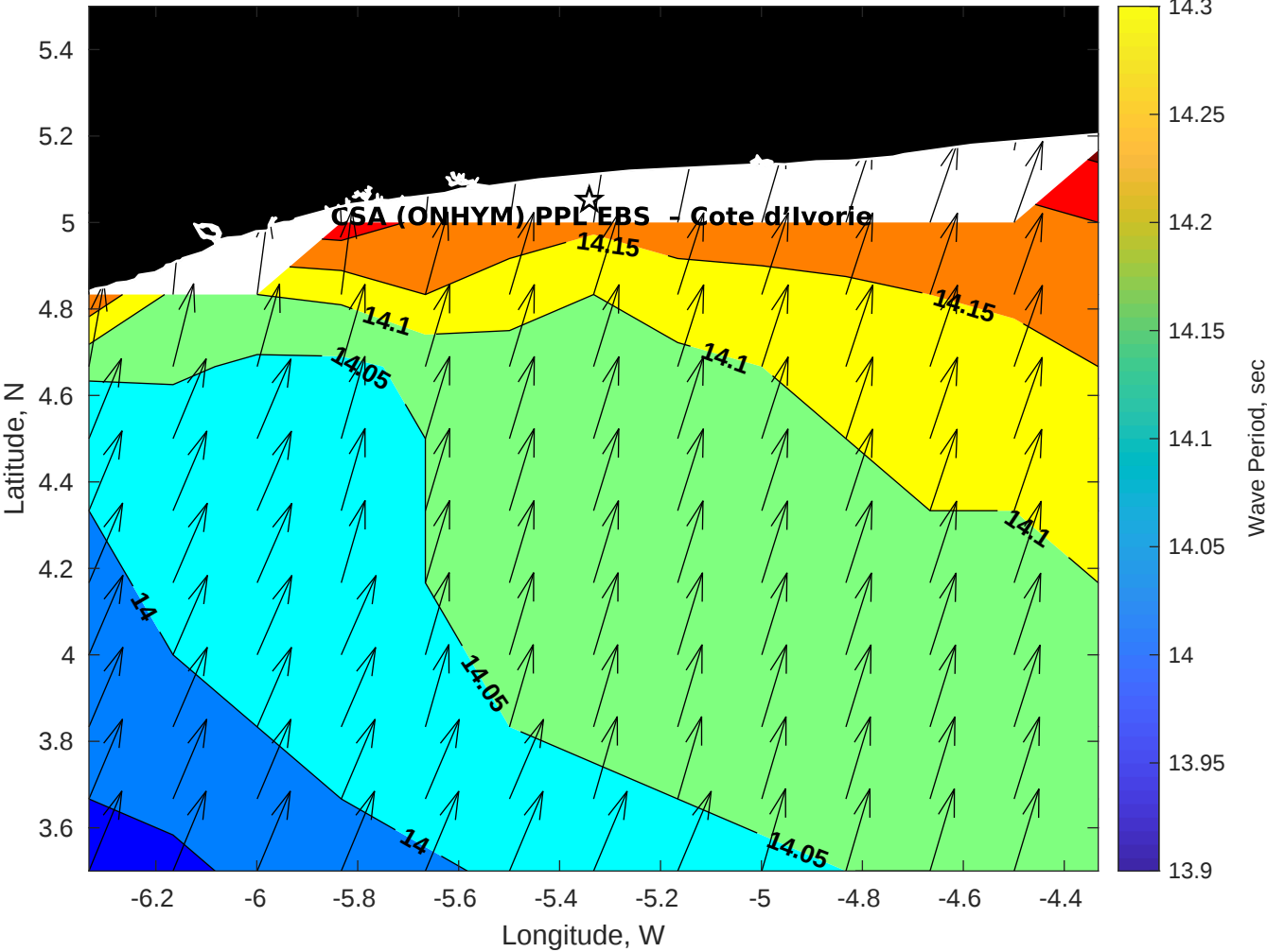
Wave Period (sec) for CSA (ONHYM) PPL EBS - Cote d'Ivoire at 13-May-2025 09:00:00
