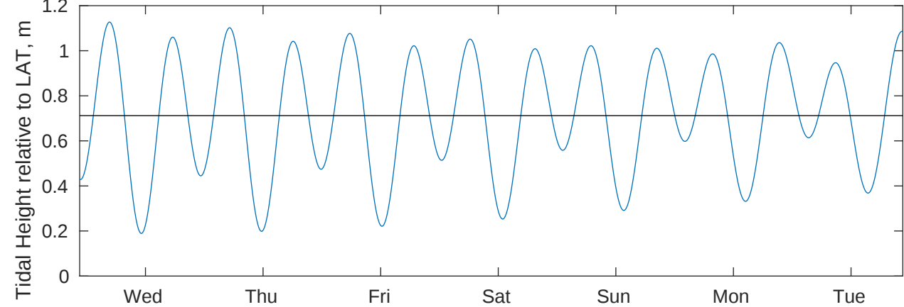
Tidal Currents and Heights for CSA (ONHYM) PPL EBS - Cote d'Ivoire at 20250513
