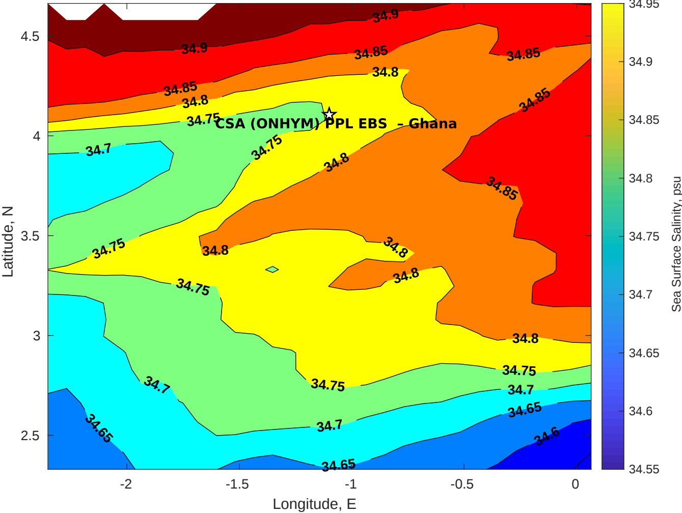
Surface Salinity for CSA (ONHYM) PPL EBS - Ghana at 12-May-2025 00:00:00
