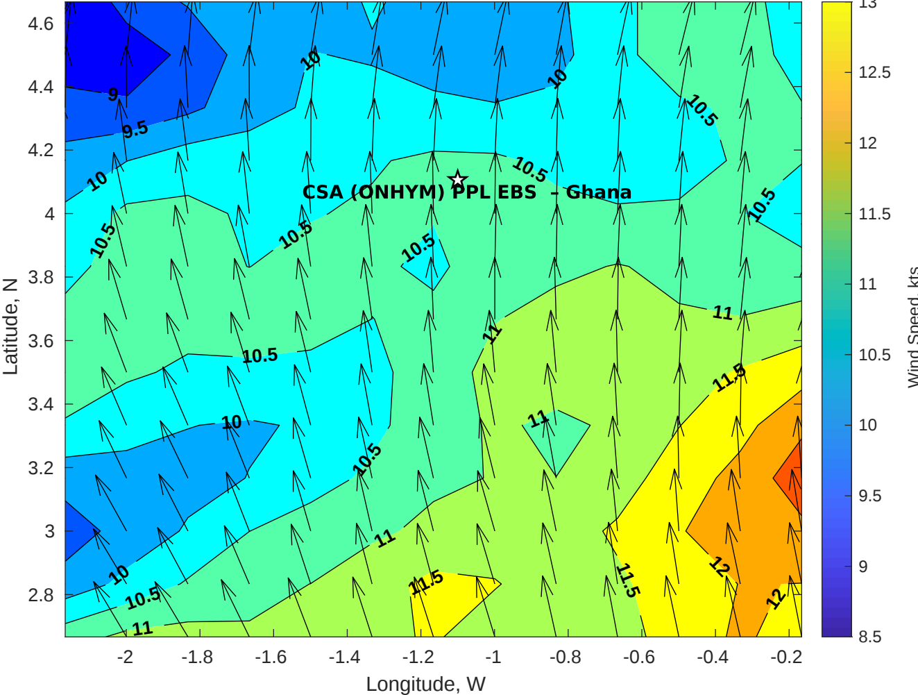
Winds (kts) for CSA (ONHYM) PPL EBS - Ghana at 13-May-2025 09:00:00
