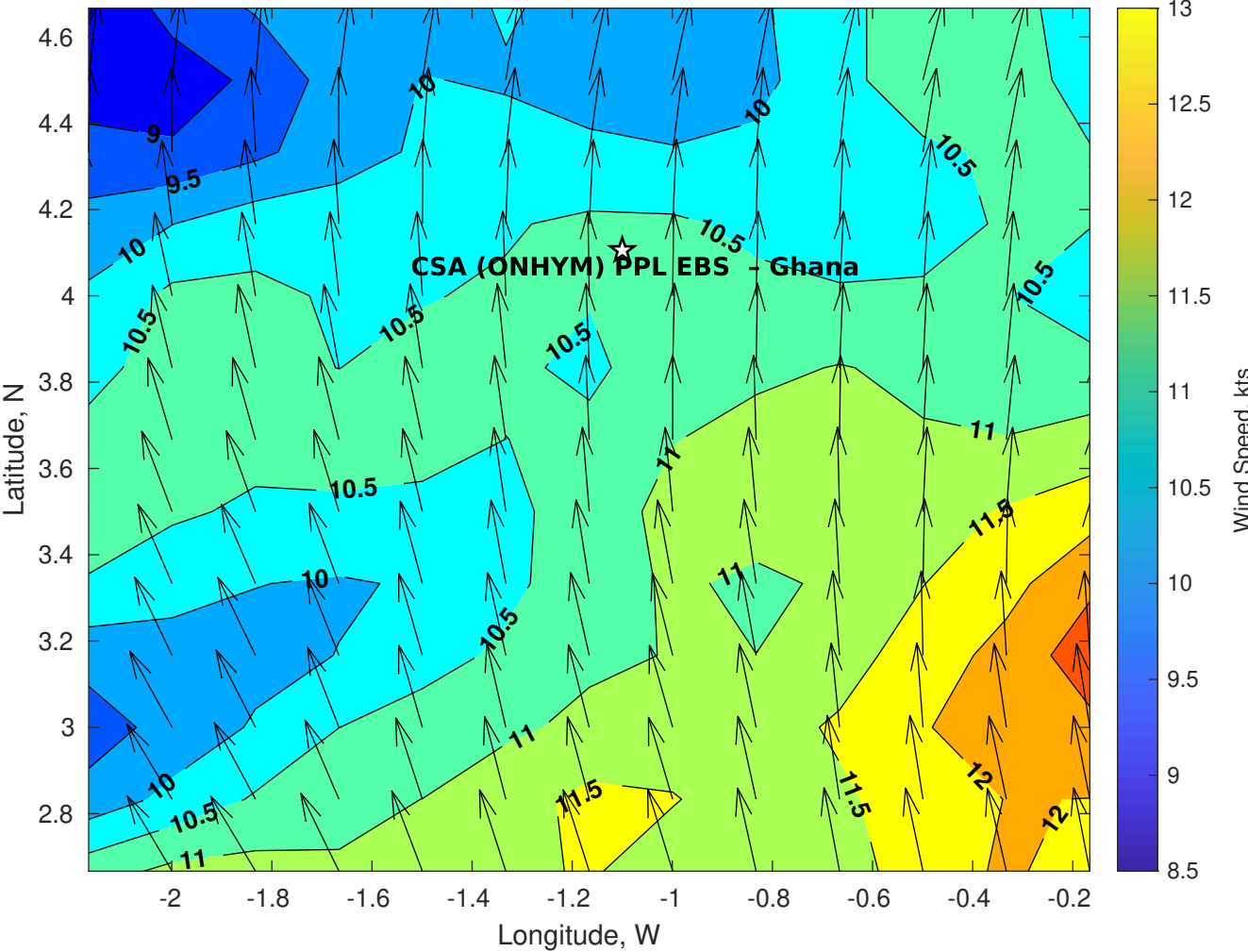
Winds (kts) for CSA (ONHYM) PPL EBS - Ghana at 13-May-2025 09:00:00
