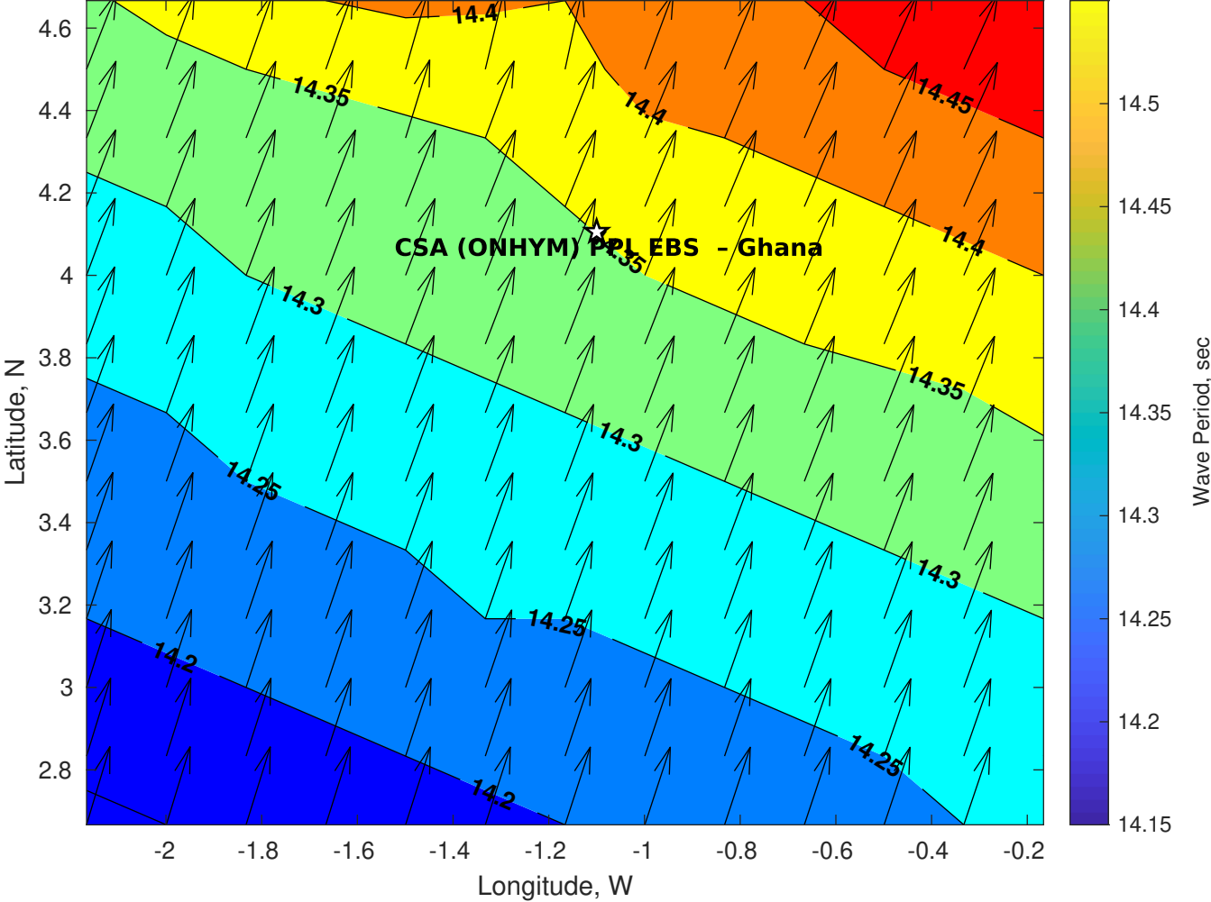
Wave Period (sec) for CSA (ONHYM) PPL EBS - Ghana at 13-May-2025 09:00:00
