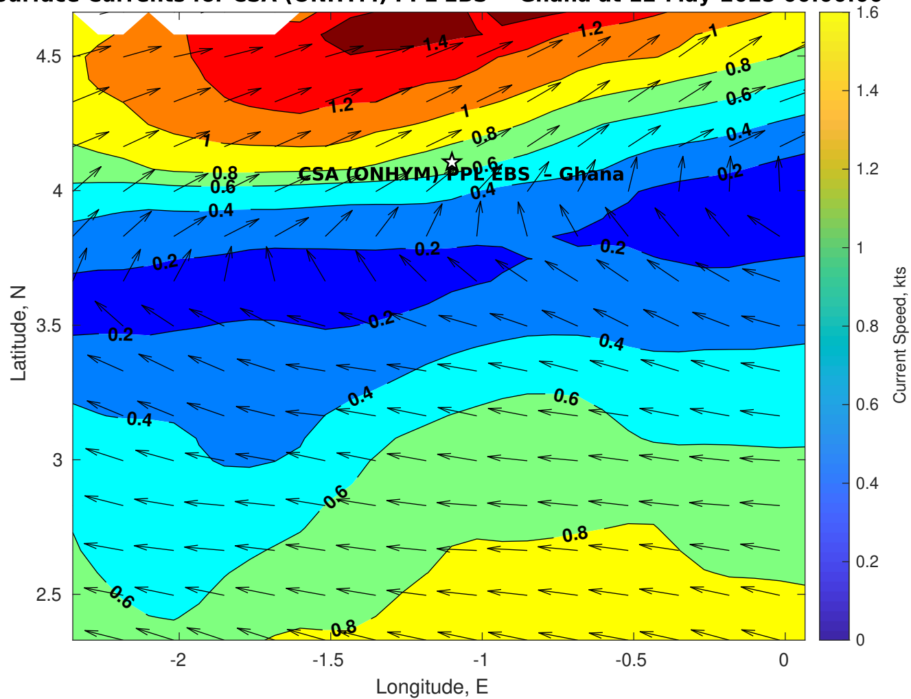
Surface Currents for CSA (ONHYM) PPL EBS - Ghana at 12-May-2025 00:00:00
