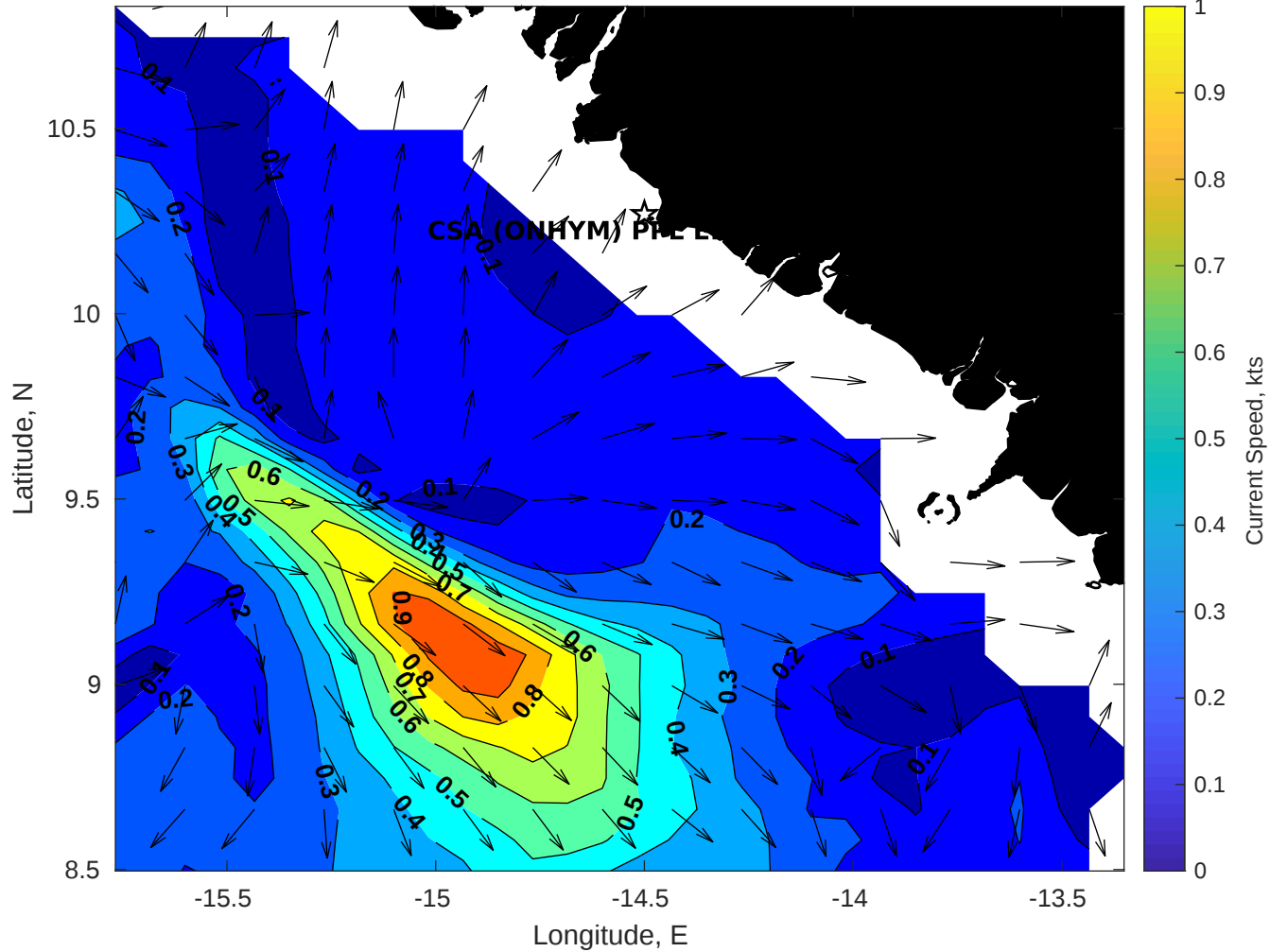
Surface Currents for CSA (ONHYM) PPL EBS - Guinea at 12-May-2025 00:00:00
