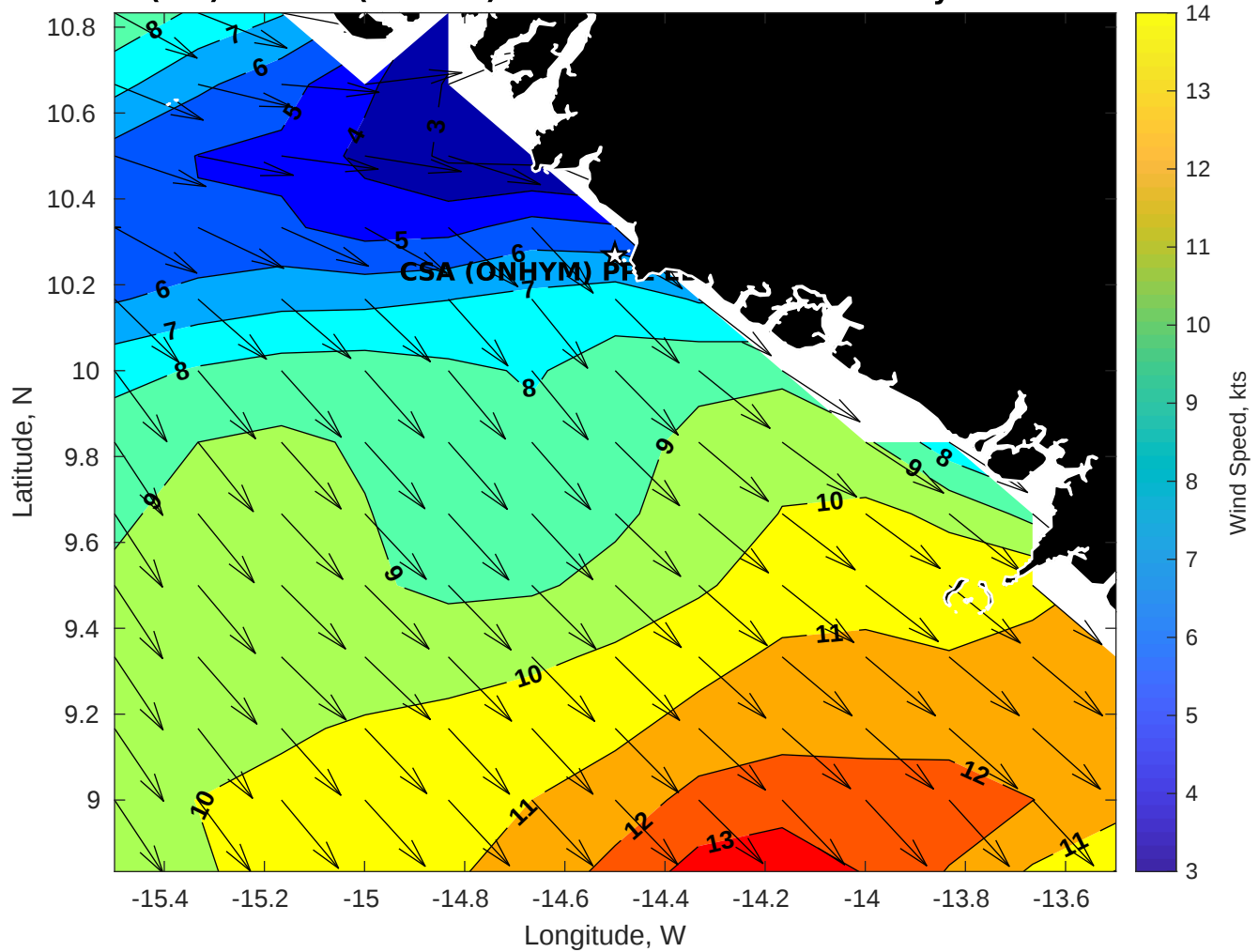
Winds (kts) for CSA (ONHYM) PPL EBS - Guinea at 13-May-2025 09:00:00
