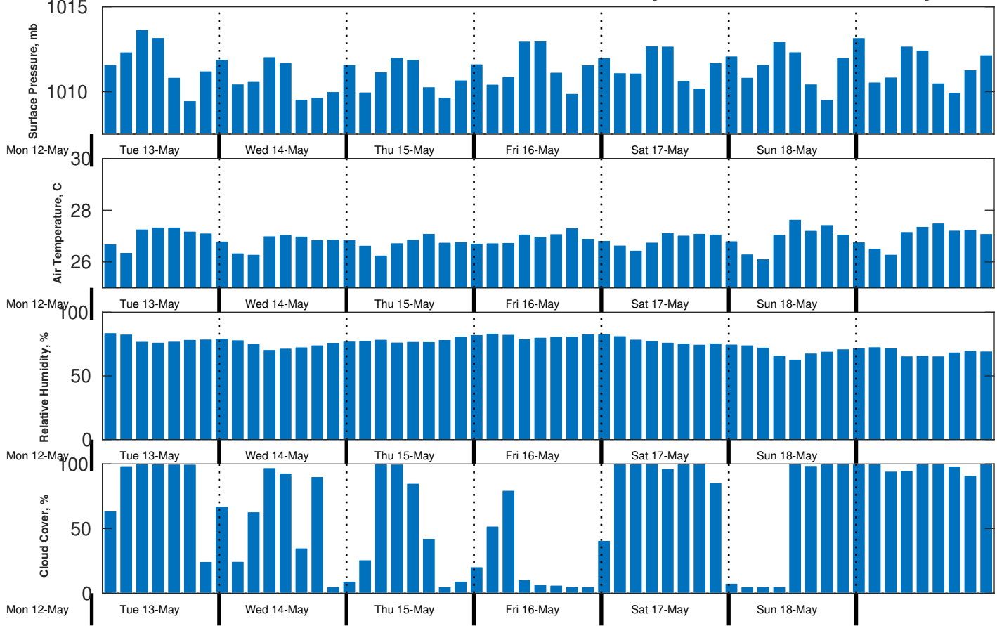
Met Forecast for CSA (ONHYM) PPL EBS - Guinea from 13-May-2025 00:00:00 to 20-May-2025 00:00:00
