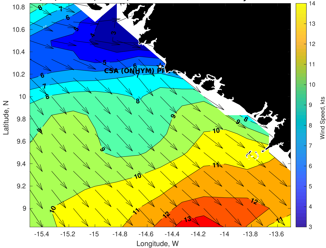
Winds (kts) for CSA (ONHYM) PPL EBS - Guinea at 13-May-2025 09:00:00
