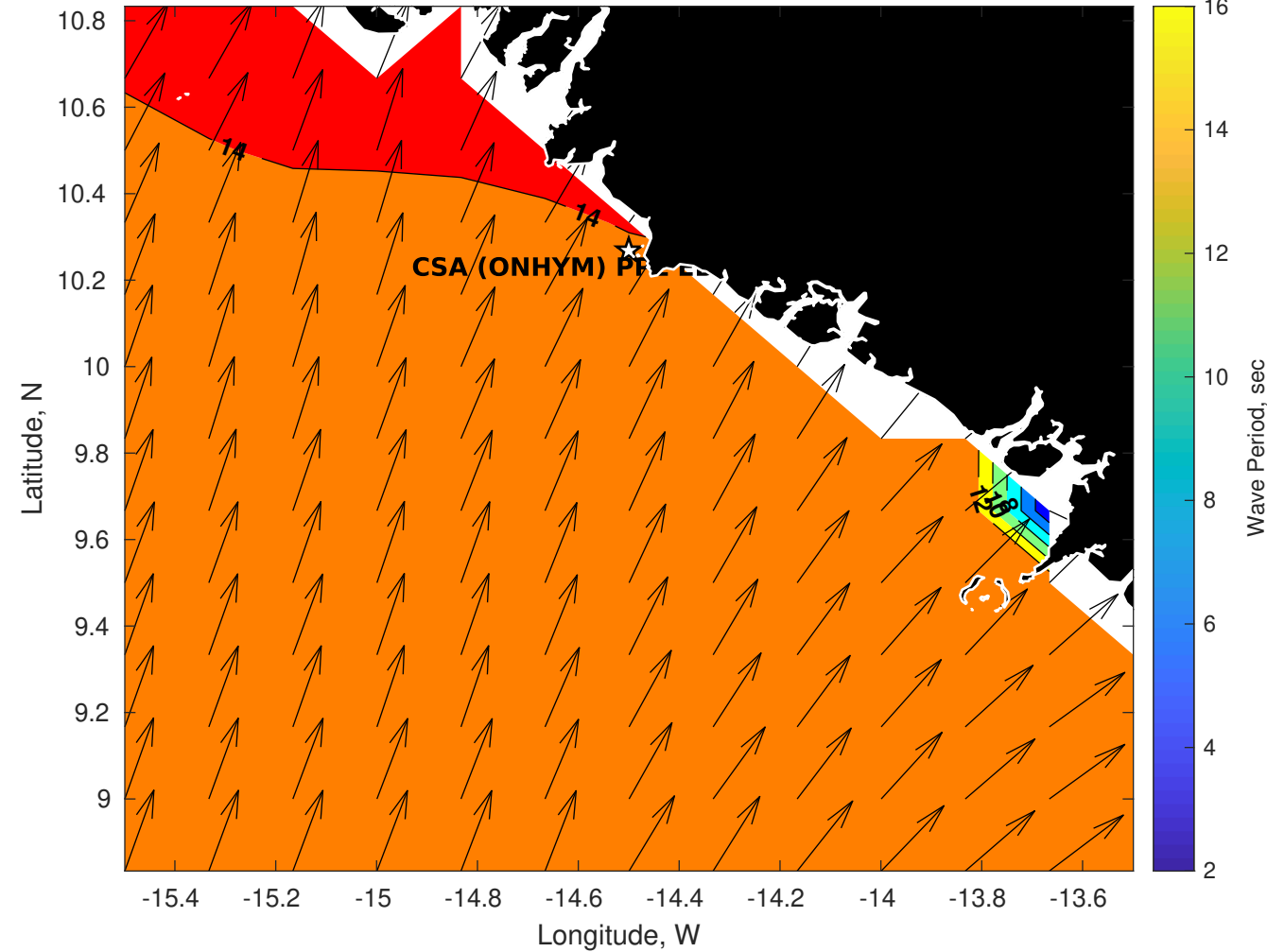
Wave Period (sec) for CSA (ONHYM) PPL EBS - Guinea at 13-May-2025 09:00:00
