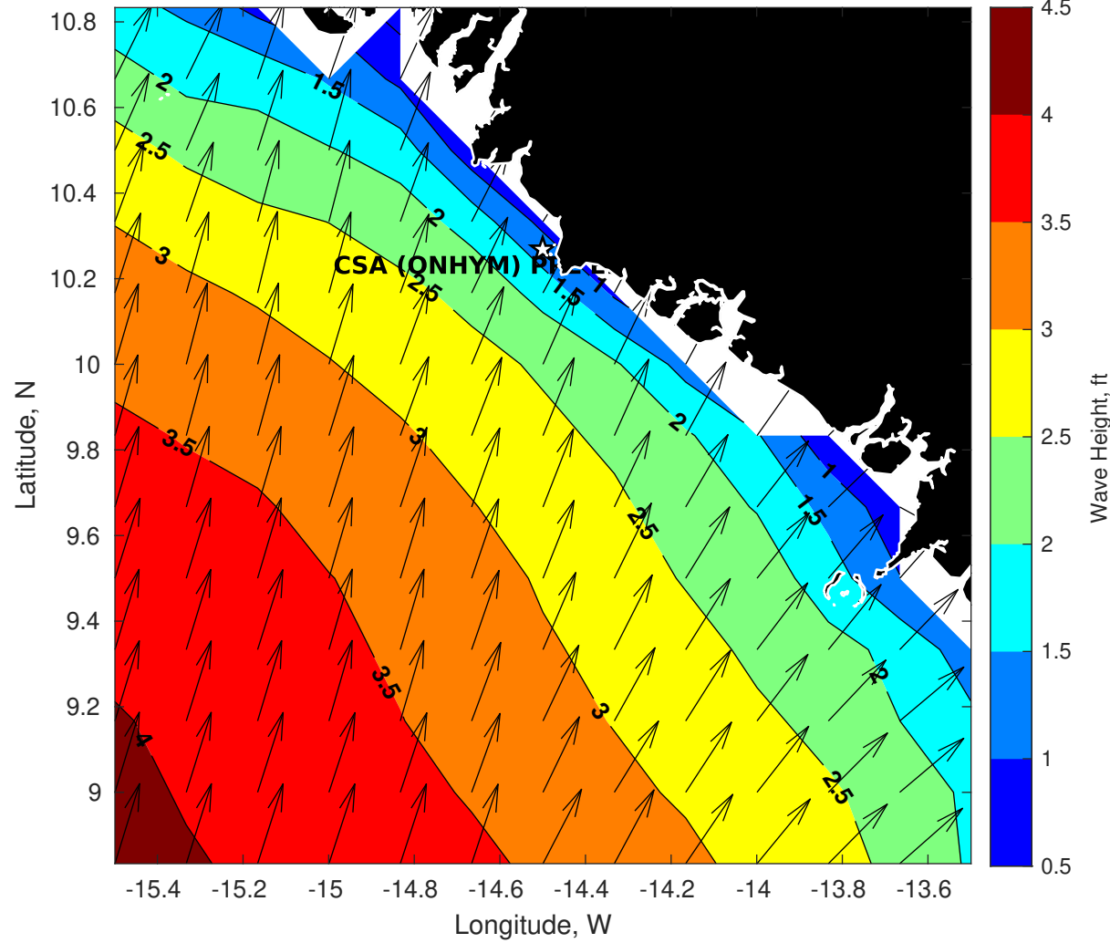
Wave Height (ft) for CSA (ONHYM) PPL EBS - Guinea at 13-May-2025 09:00:00
