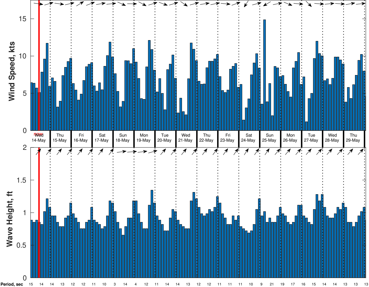
Wind & Wave Forecast for CSA (ONHYM) PPL EBS - Guinea from 13-May-2025 01:00:00 to 29-May-2025 01:00:00
