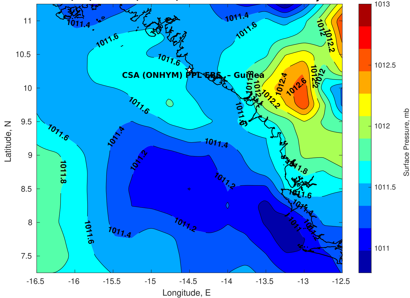
Surface Pressure (mb) for CSA (ONHYM) PPL EBS - Guinea at 15-May-2025 00:00:00
