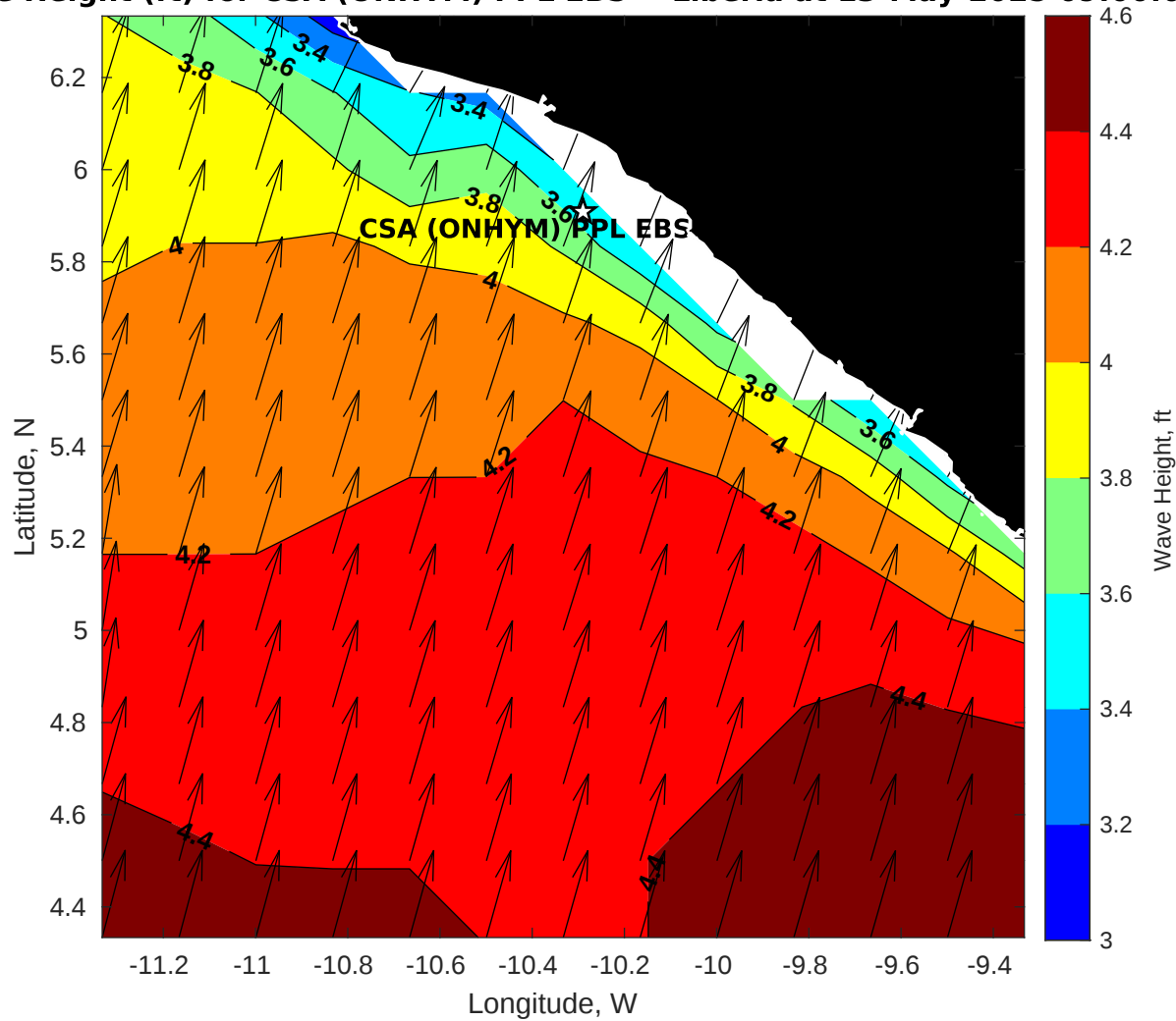
Wave Height (ft) for CSA (ONHYM) PPL EBS - Liberia at 13-May-2025 09:00:00
