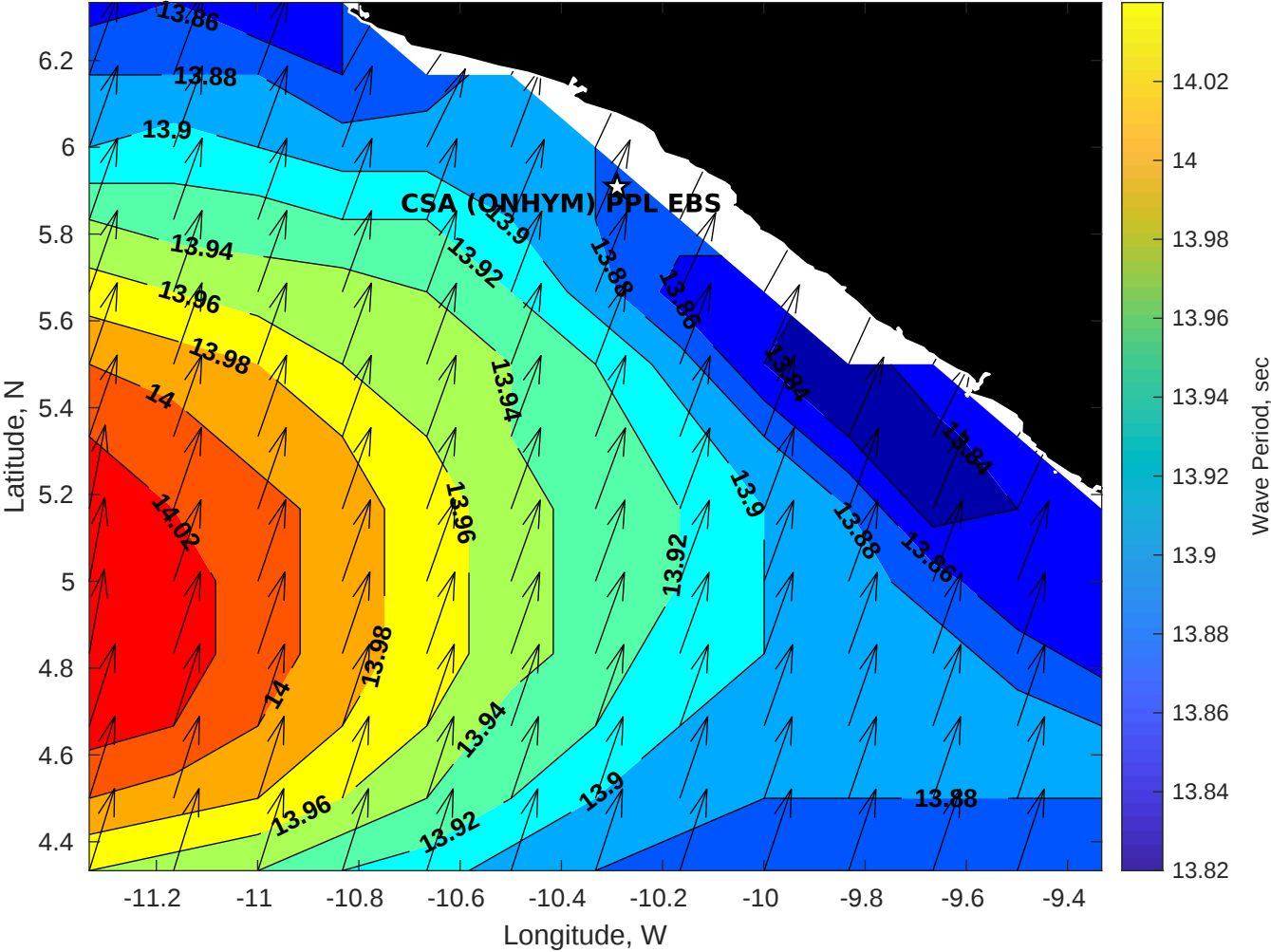
Wave Period (sec) for CSA (ONHYM) PPL EBS - Liberia at 13-May-2025 09:00:00
