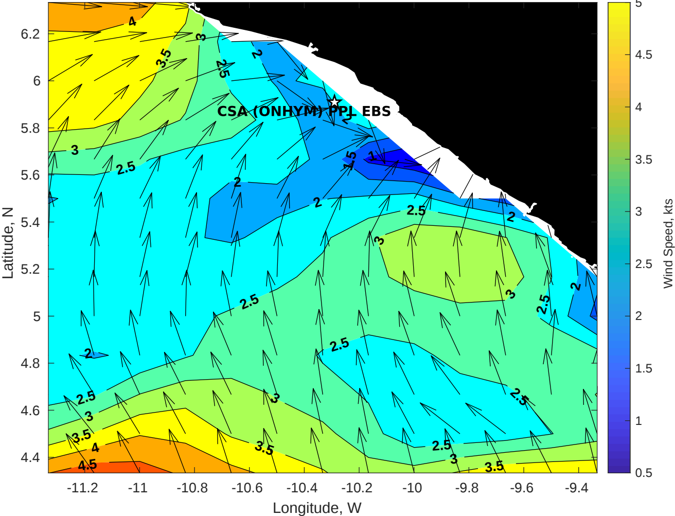
Winds (kts) for CSA (ONHYM) PPL EBS - Liberia at 13-May-2025 09:00:00
