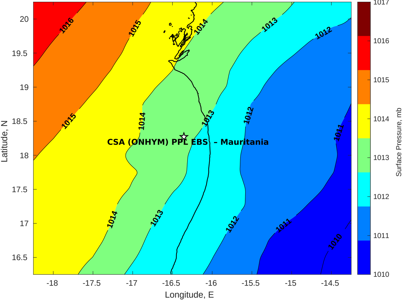
Surface Pressure (mb) for CSA (ONHYM) PPL EBS - Mauritania at 13-May-2025 00:00:00
