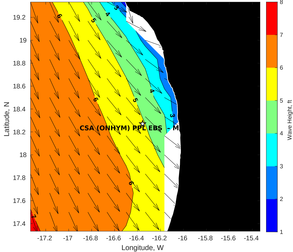
Wave Height (ft) for CSA (ONHYM) PPL EBS - Mauritania at 13-May-2025 09:00:00
