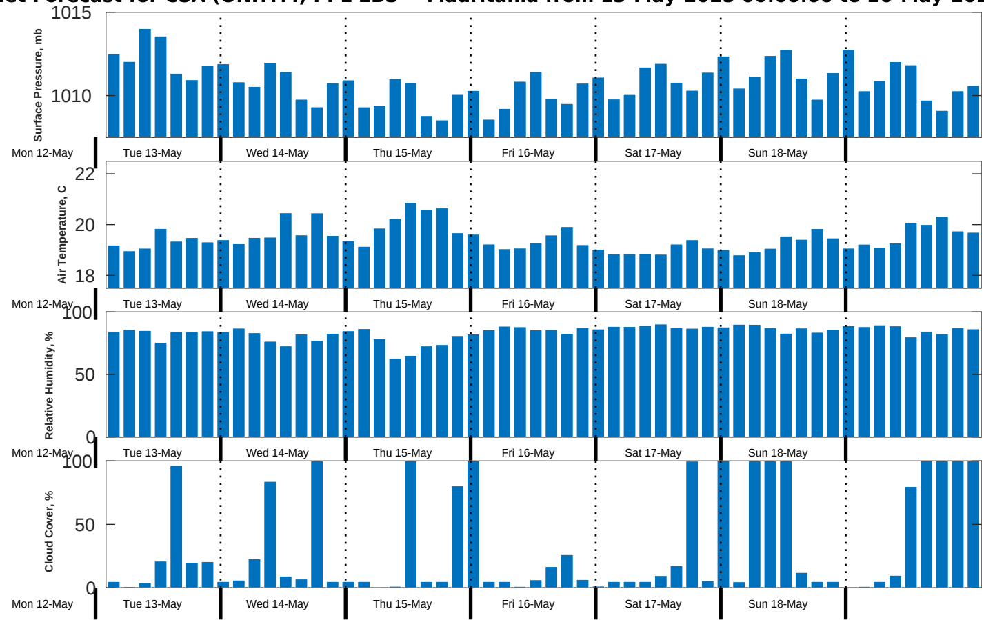
Met Forecast for CSA (ONHYM) PPL EBS - Mauritania from 13-May-2025 00:00:00 to 20-May-2025 00:00:00
