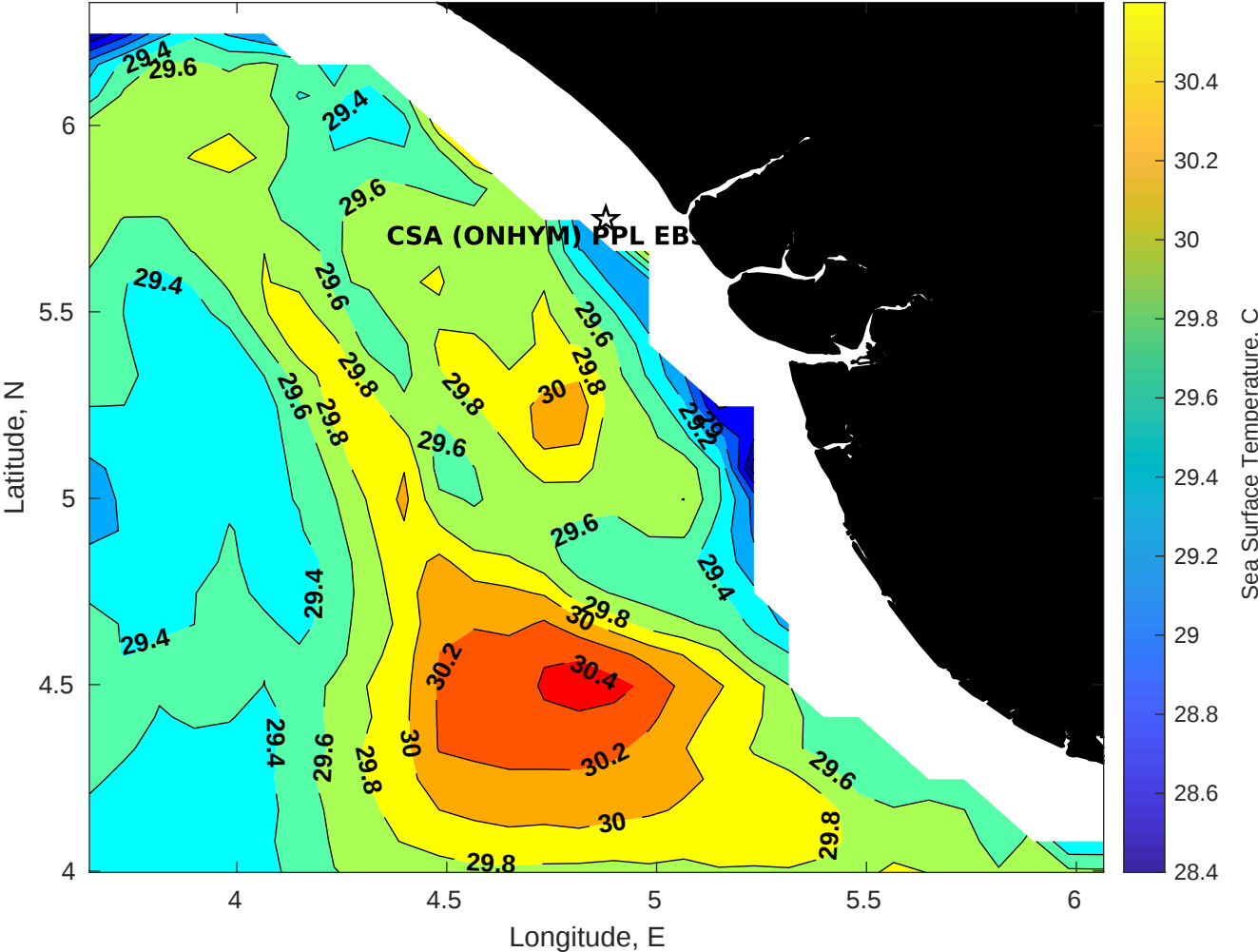
SST for CSA (ONHYM) PPL EBS - Nigeria at 12-May-2025 00:00:00
