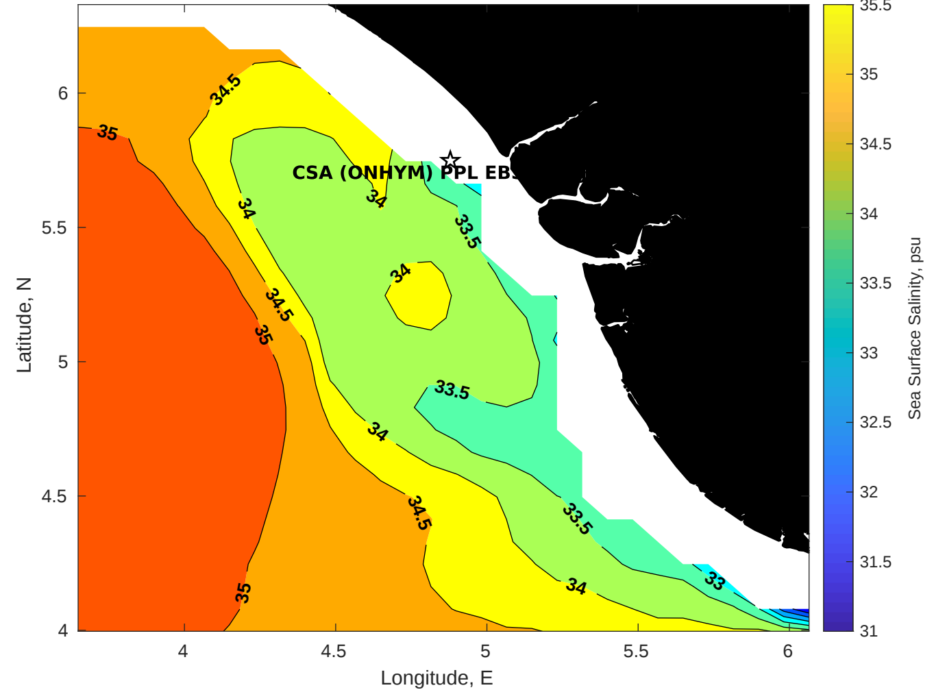
Surface Salinity for CSA (ONHYM) PPL EBS - Nigeria at 12-May-2025 00:00:00
