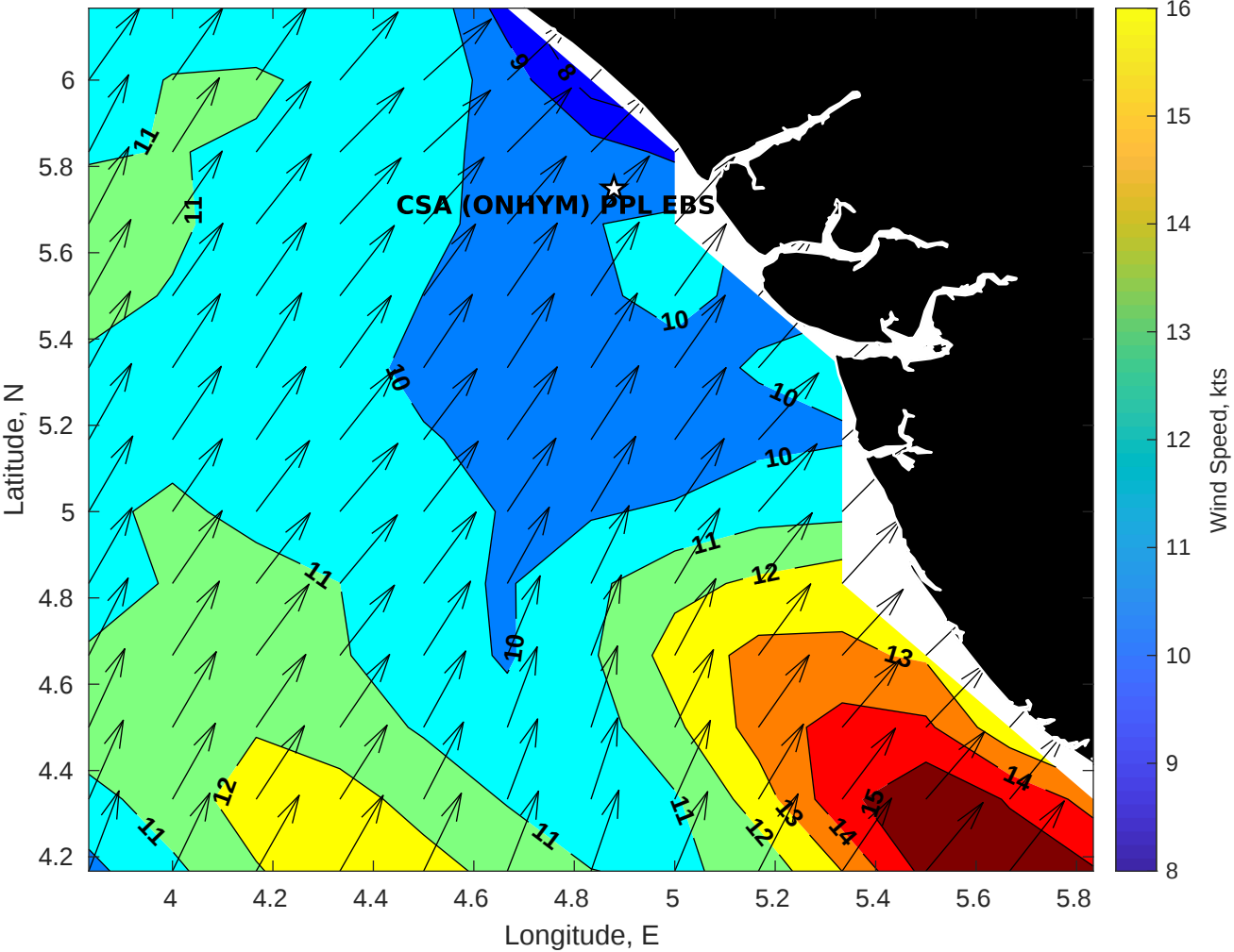
Winds (kts) for CSA (ONHYM) PPL EBS - Nigeria at 13-May-2025 09:00:00
