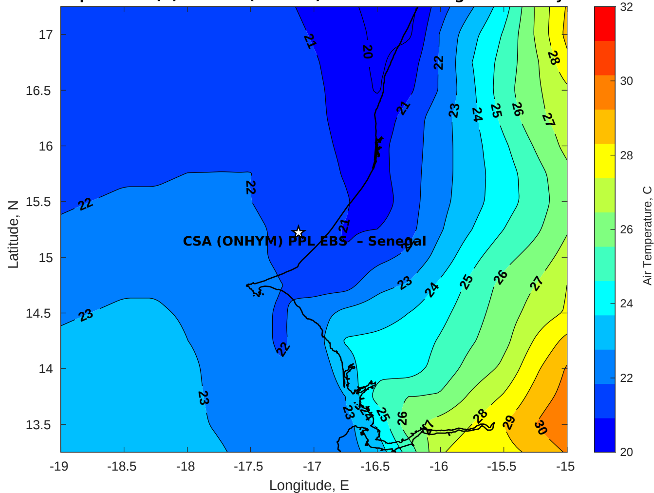
Air Temperature (C) for CSA (ONHYM) PPL EBS - Senegal at 13-May-2025
