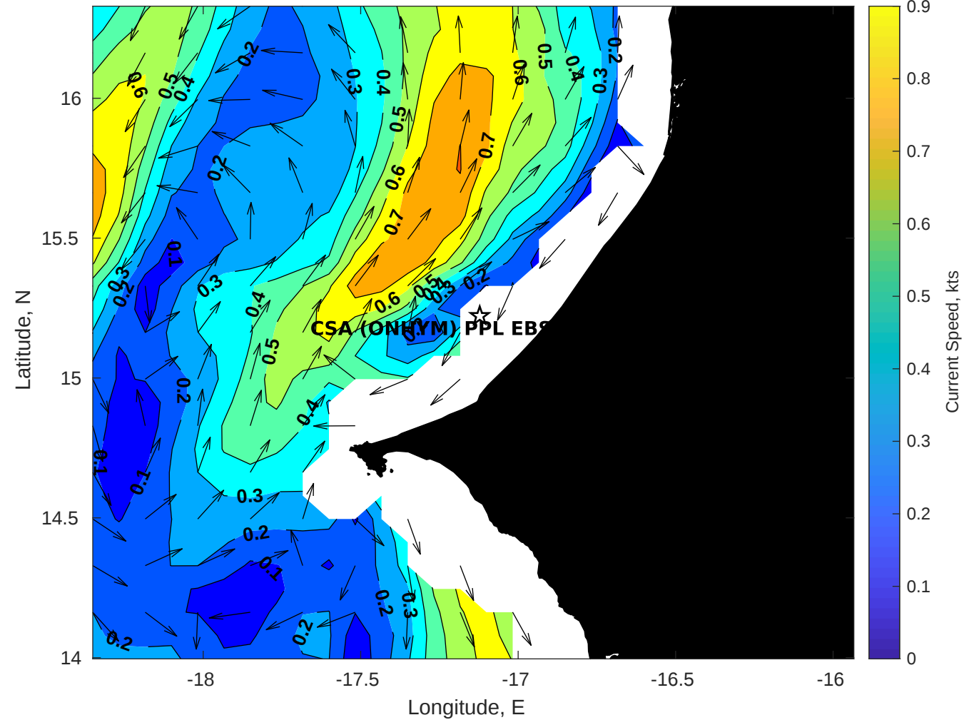
Surface Currents for CSA (ONHYM) PPL EBS - Senegal at 12-May-2025 00:00:00
