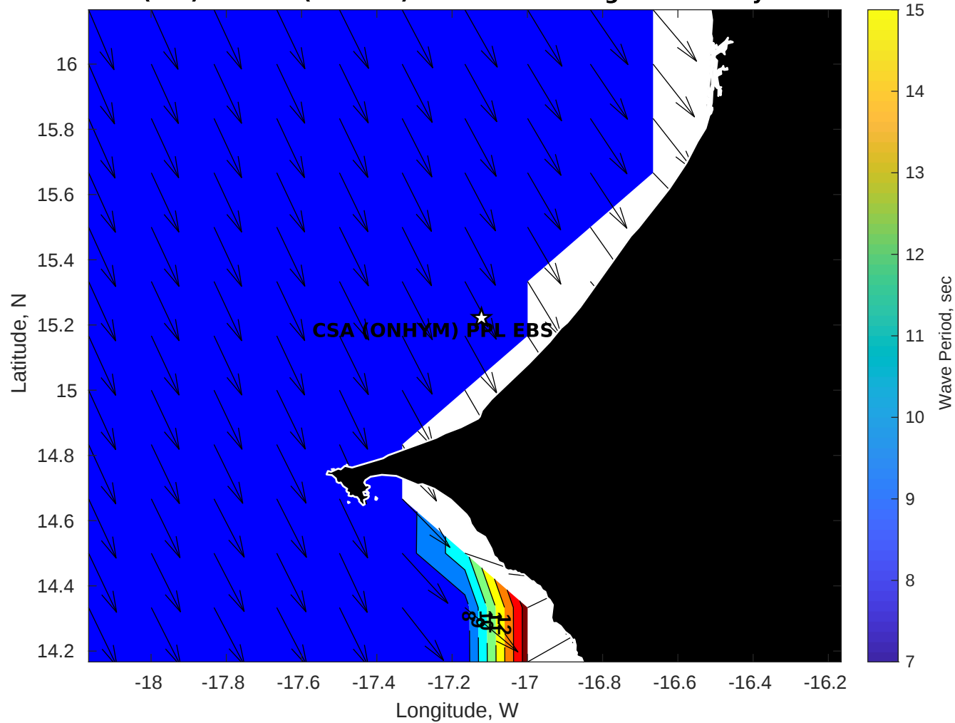
Wave Period (sec) for CSA (ONHYM) PPL EBS - Senegal at 13-May-2025 09:00:00
