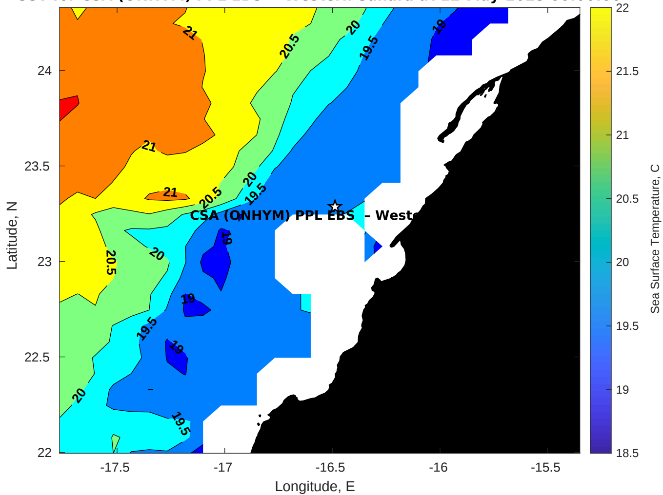
SST for CSA (ONHYM) PPL EBS - Western Sahara at 12-May-2025 00:00:00
