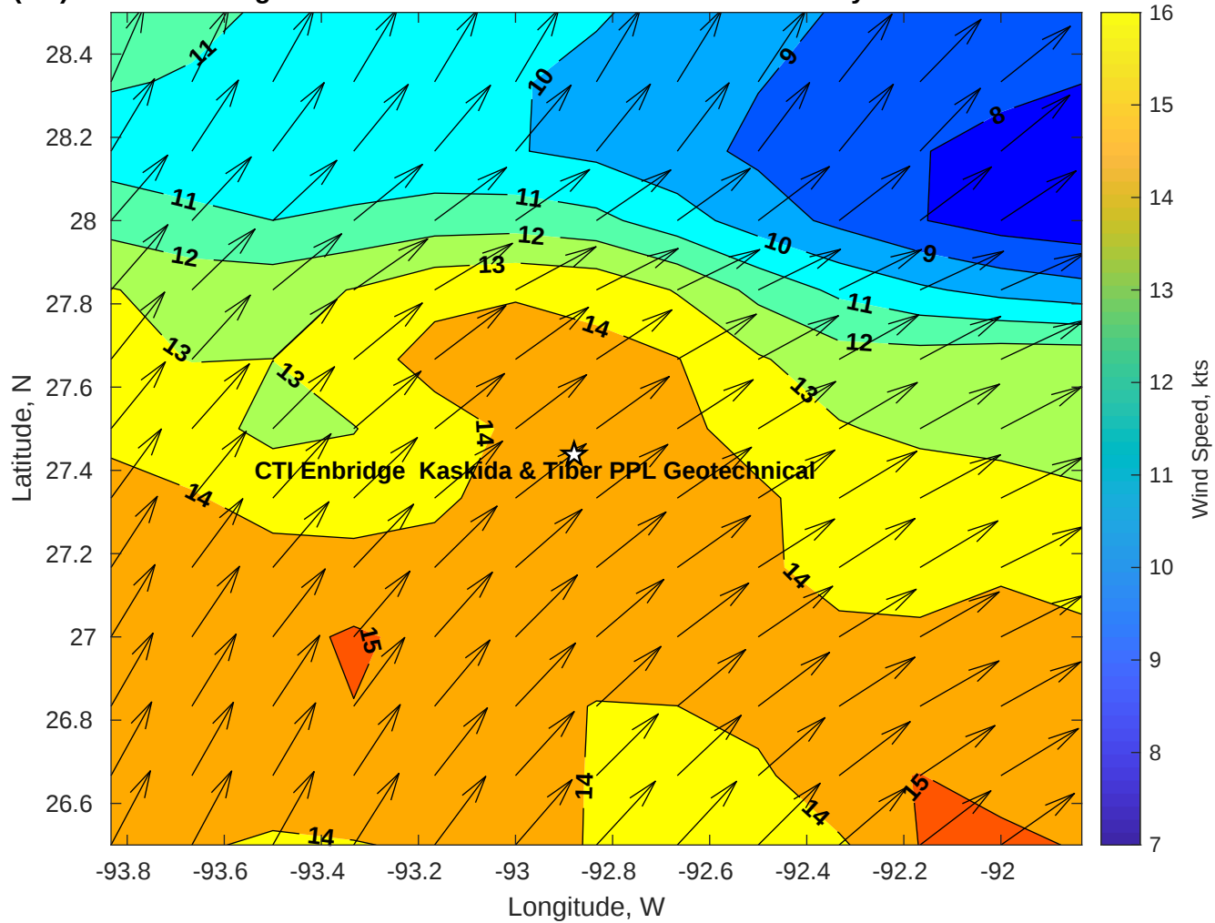
Winds (kts) for CTI Enbridge Kaskida & Tiber PPL Geotechnical at 13-May-2025 09:00:00
