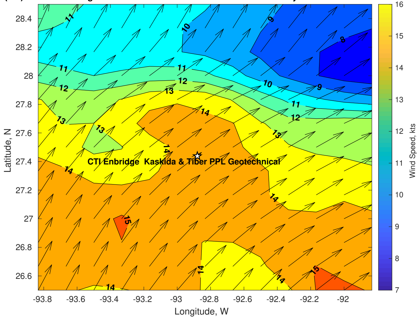
Winds (kts) for CTI Enbridge Kaskida & Tiber PPL Geotechnical at 13-May-2025 09:00:00
