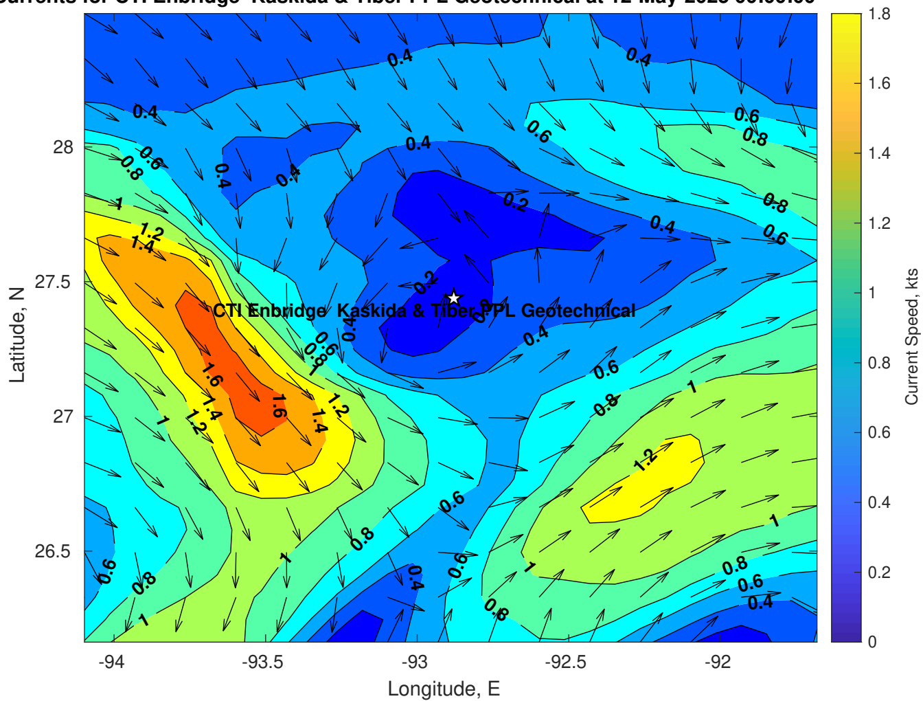
Surface Currents for CTI Enbridge Kaskida & Tiber PPL Geotechnical at 12-May-2025 00:00:00
