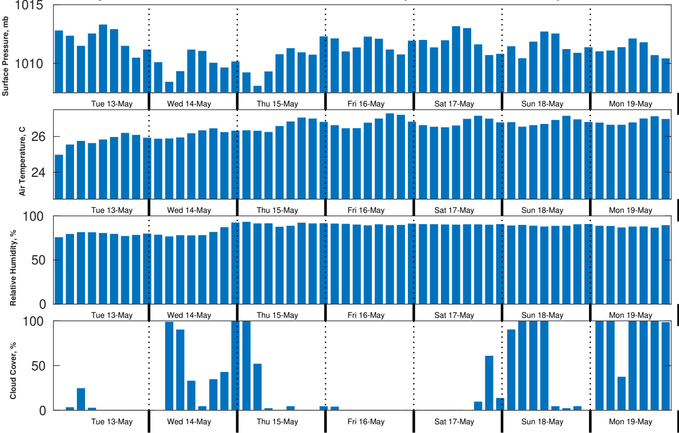
Met Forecast for CTI Enbridge Kaskida & Tiber PPL Geotechnical from 13-May-2025 00:00:00 to 20-May-2025 00:00:00
