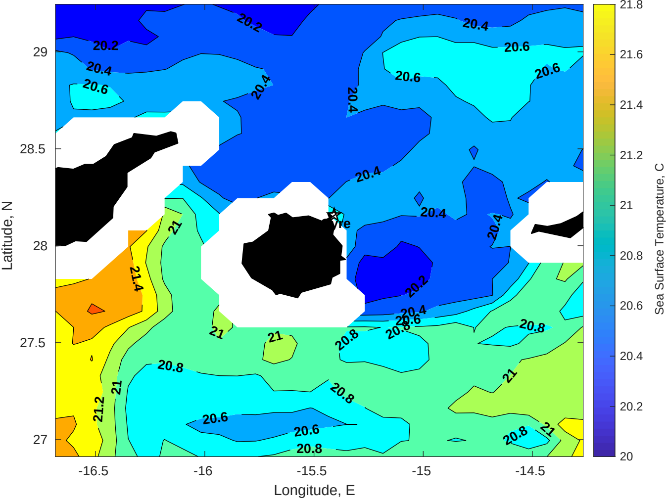
SST for Gyre at 12-May-2025 00:00:00
