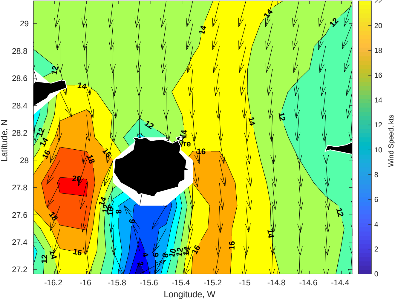
Winds (kts) for Gyre at 13-May-2025 09:00:00
