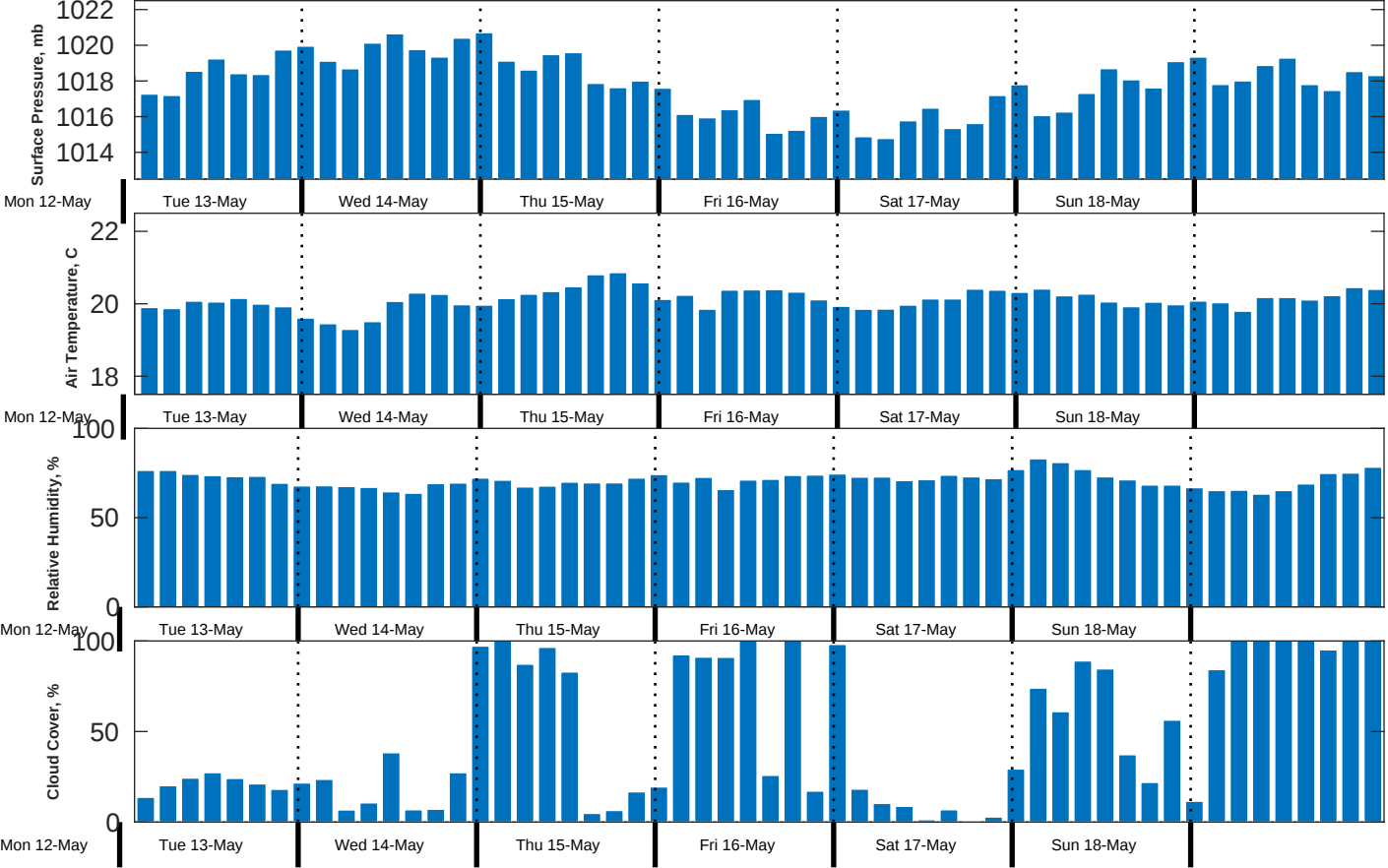
Met Forecast for Gyre from 12-May-2025 23:00:00 to 19-May-2025 23:00:00
