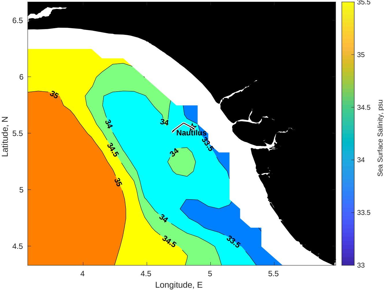
Surface Salinity for Nautilus at 12-May-2025 00:00:00
