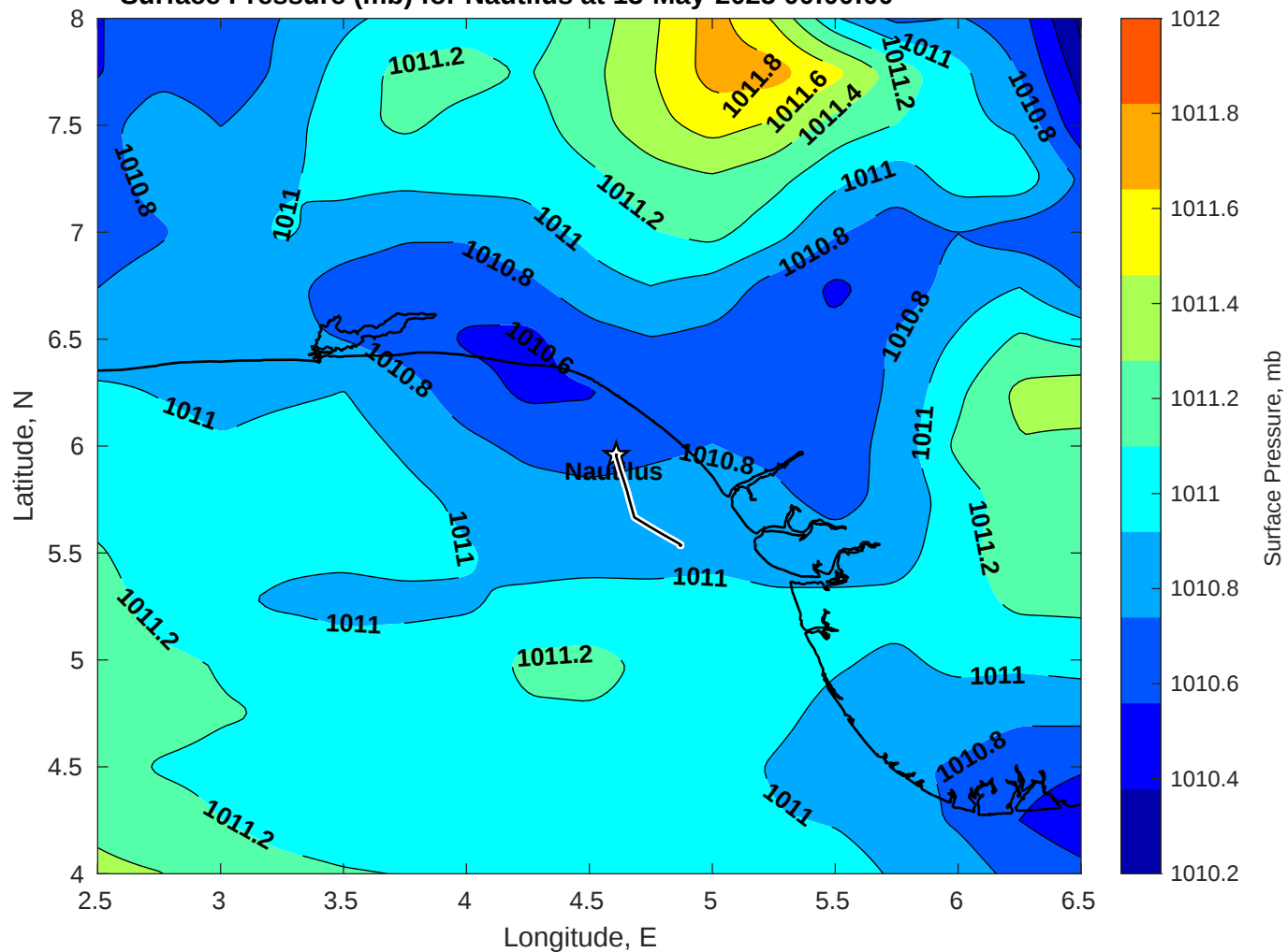
Surface Pressure (mb) for Nautilus at 13-May-2025 00:00:00
