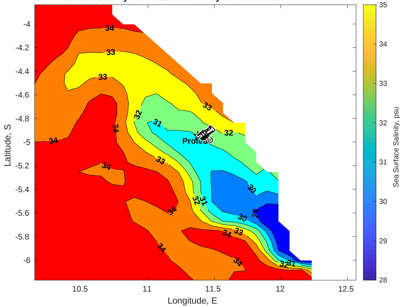
Surface Salinity for Proteus at 12-May-2025 00:00:00
