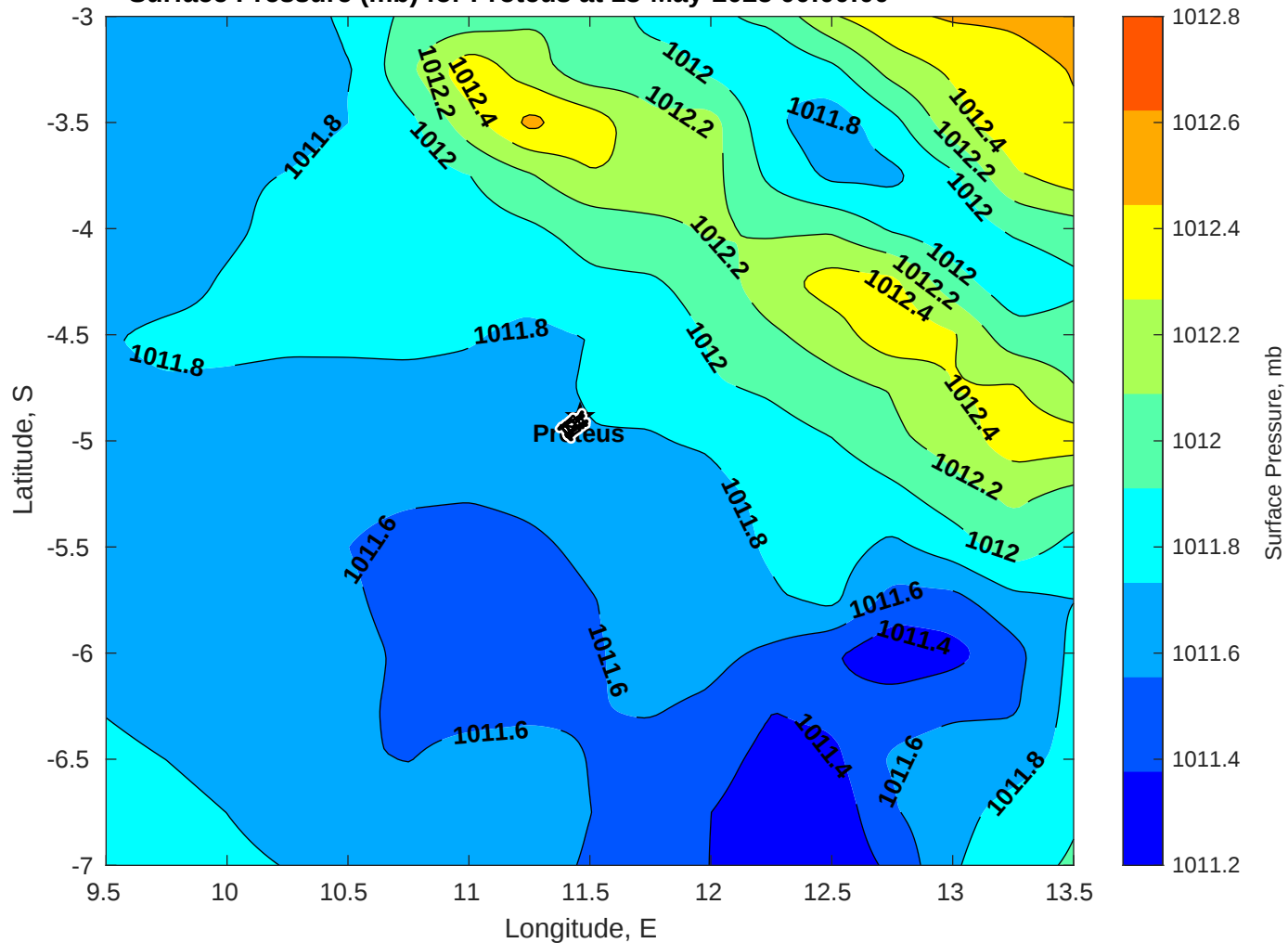
Surface Pressure (mb) for Proteus at 13-May-2025 00:00:00
