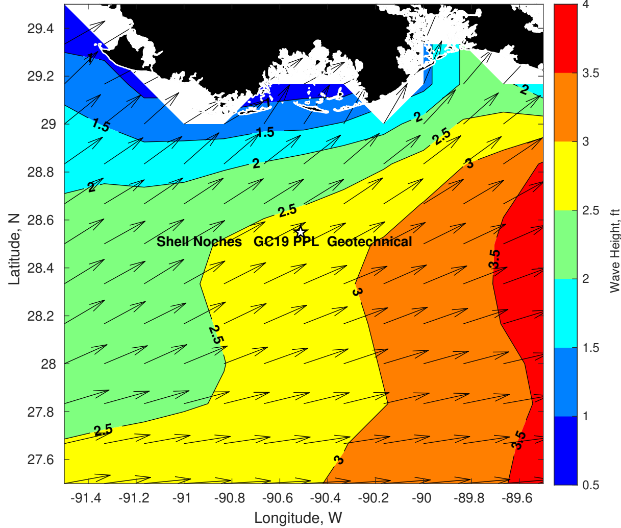
Wave Height (ft) for Shell Noches GC19 PPL Geotechnical at 13-May-2025 09:00:00
