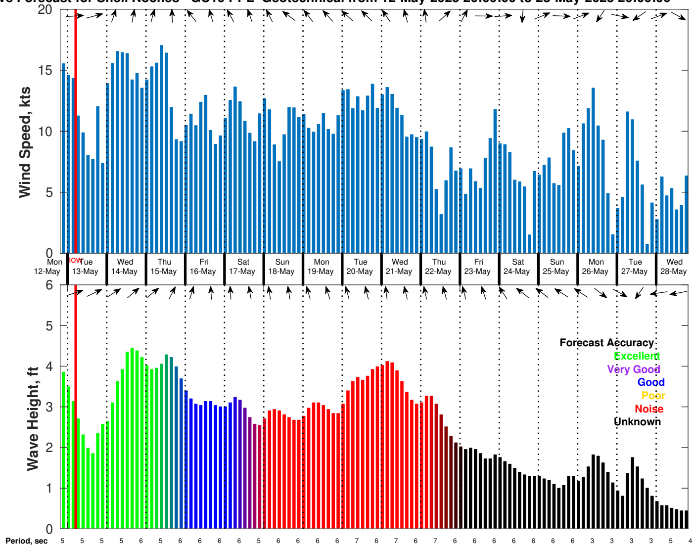
Wind & Wave Forecast for Shell Noches GC19 PPL Geotechnical from 12-May-2025 20:00:00 to 28-May-2025 20:00:00
