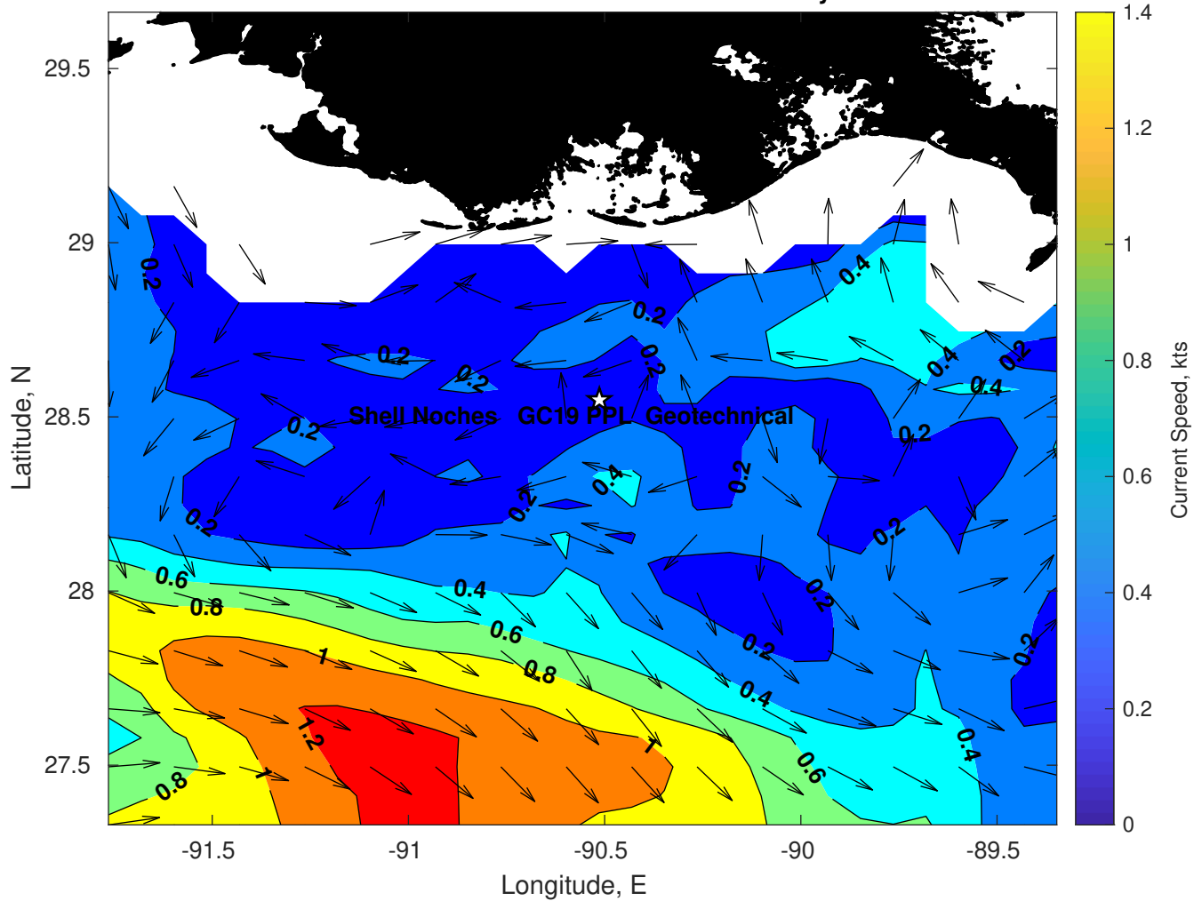
Surface Currents for Shell Noches GC19 PPL Geotechnical at 12-May-2025 00:00:00
