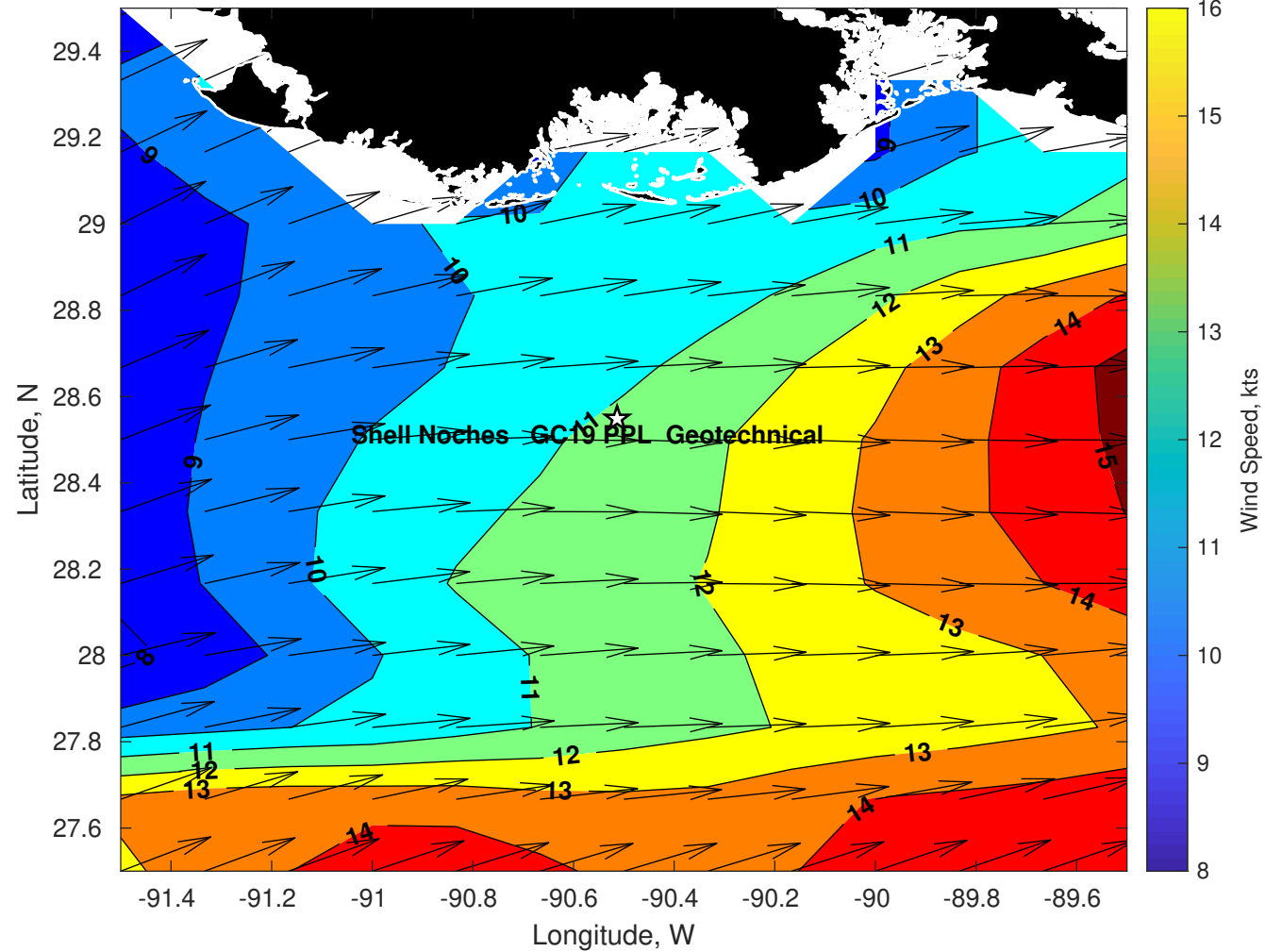
Winds (kts) for Shell Noches GC19 PPL Geotechnical at 13-May-2025 09:00:00
