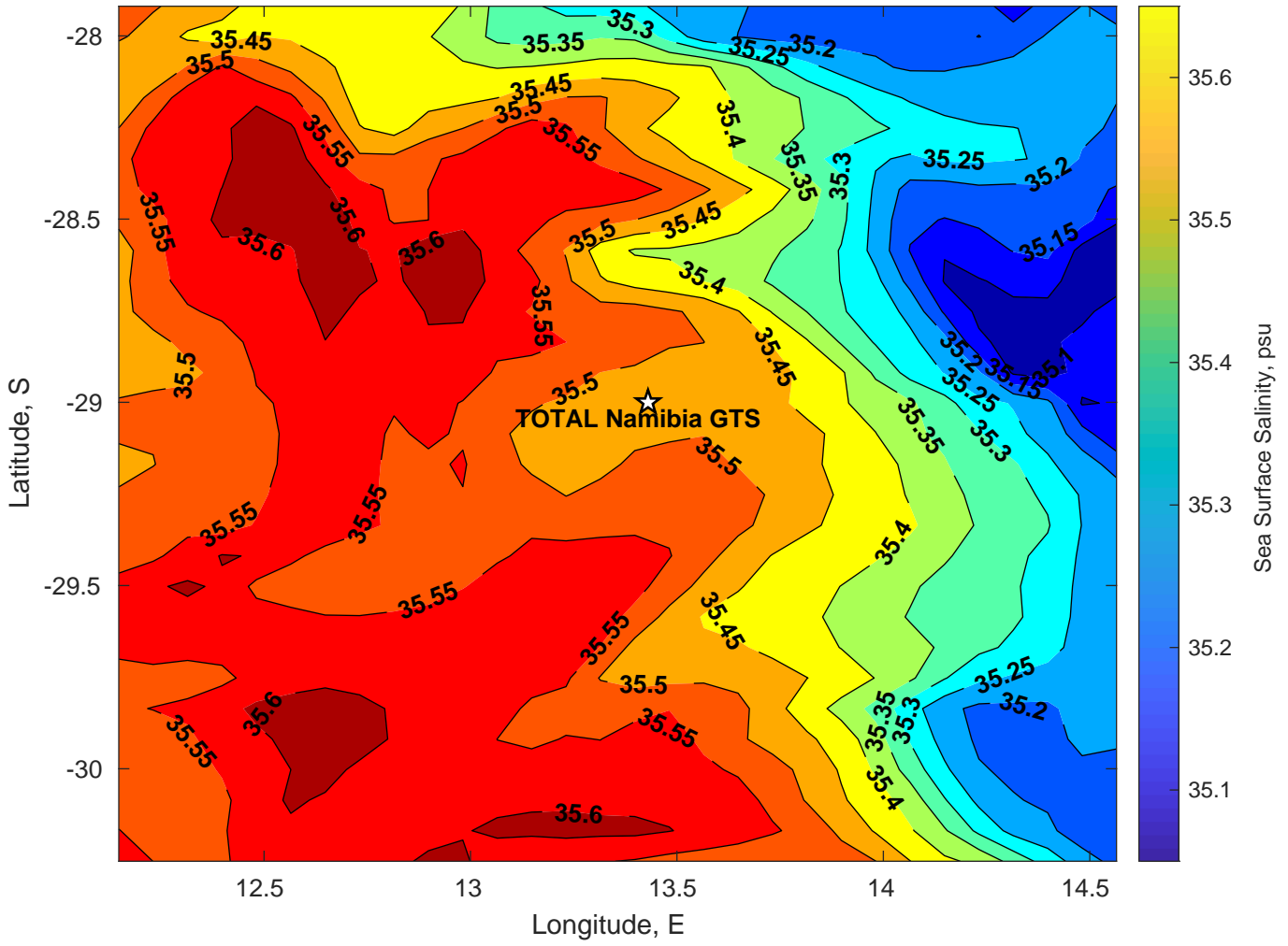
Surface Salinity for TOTAL Namibia GTS at 12-May-2025 00:00:00
