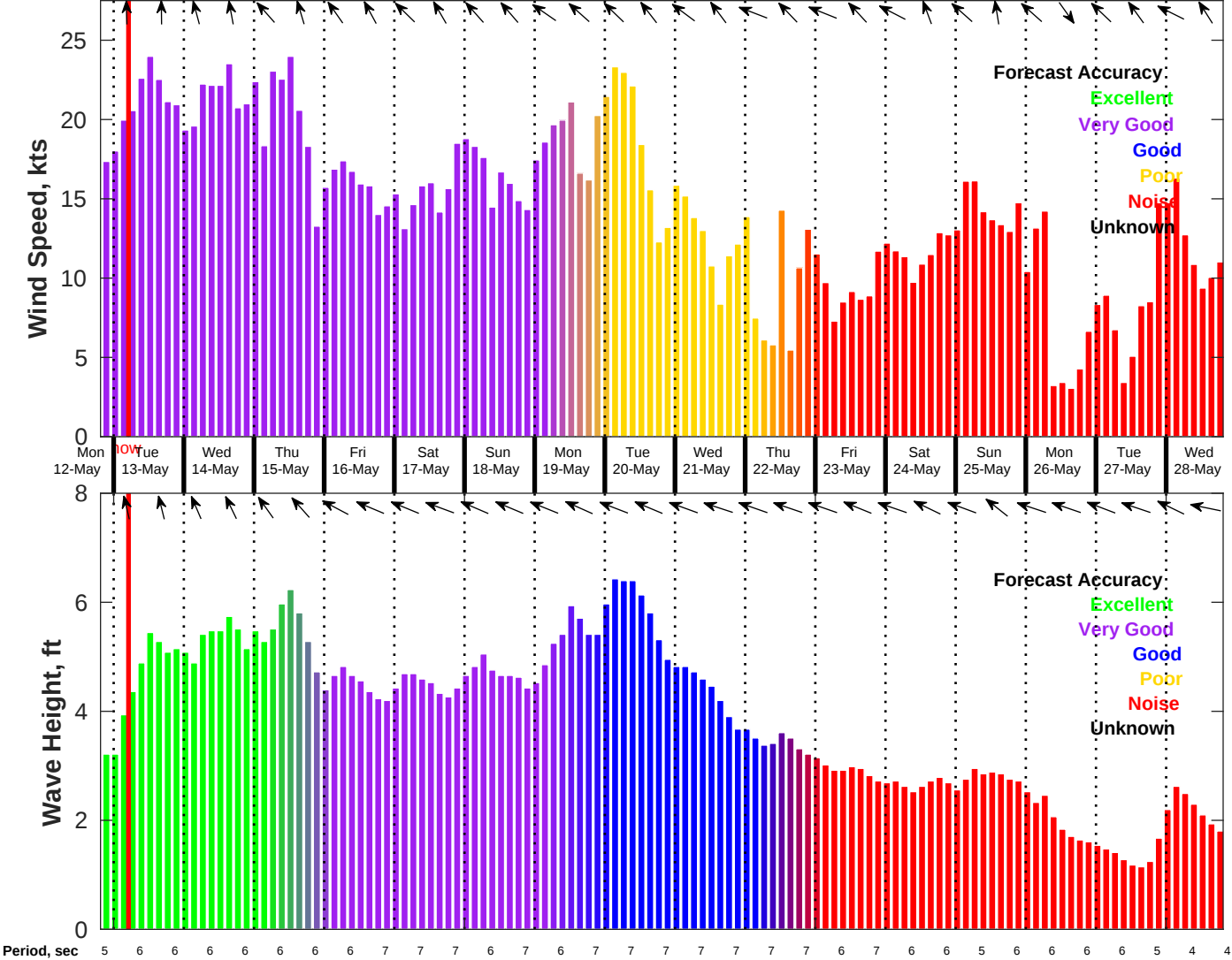
Wind & Wave Forecast for Tampnet P2378 South Texas Cable Route Geophysical from 12-May-2025 20:00:00 to 28-May-2025 20:00:00
