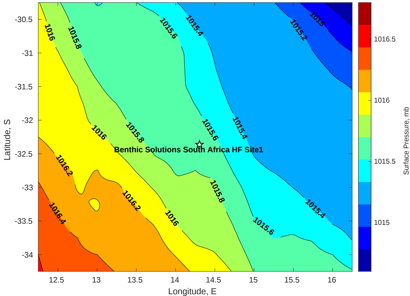
Surface Pressure (mb) for Benthic Solutions South Africa HF Site1 at 16-May-2025 00:00:00
