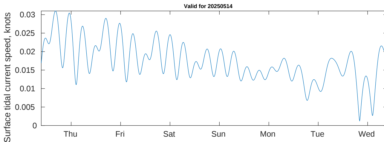
Tidal Currents and Heights for Benthic Solutions South Africa HF Site1 at 20250514
