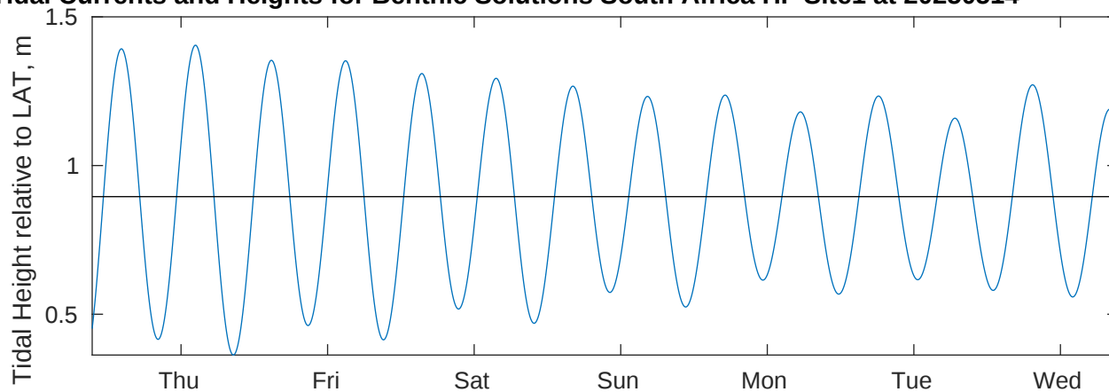
Tidal Currents and Heights for Benthic Solutions South Africa HF Site1 at 20250514
