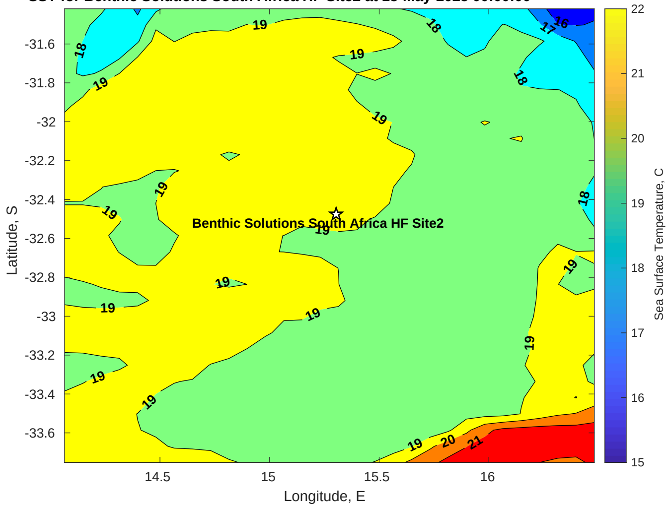
SST for Benthic Solutions South Africa HF Site2 at 13-May-2025 00:00:00
