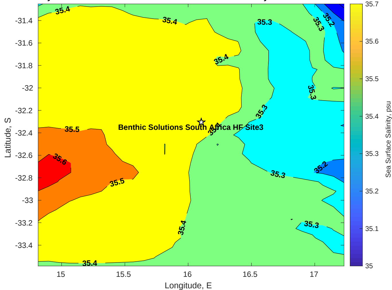
Surface Salinity for Benthic Solutions South Africa HF Site3 at 13-May-2025 00:00:00
