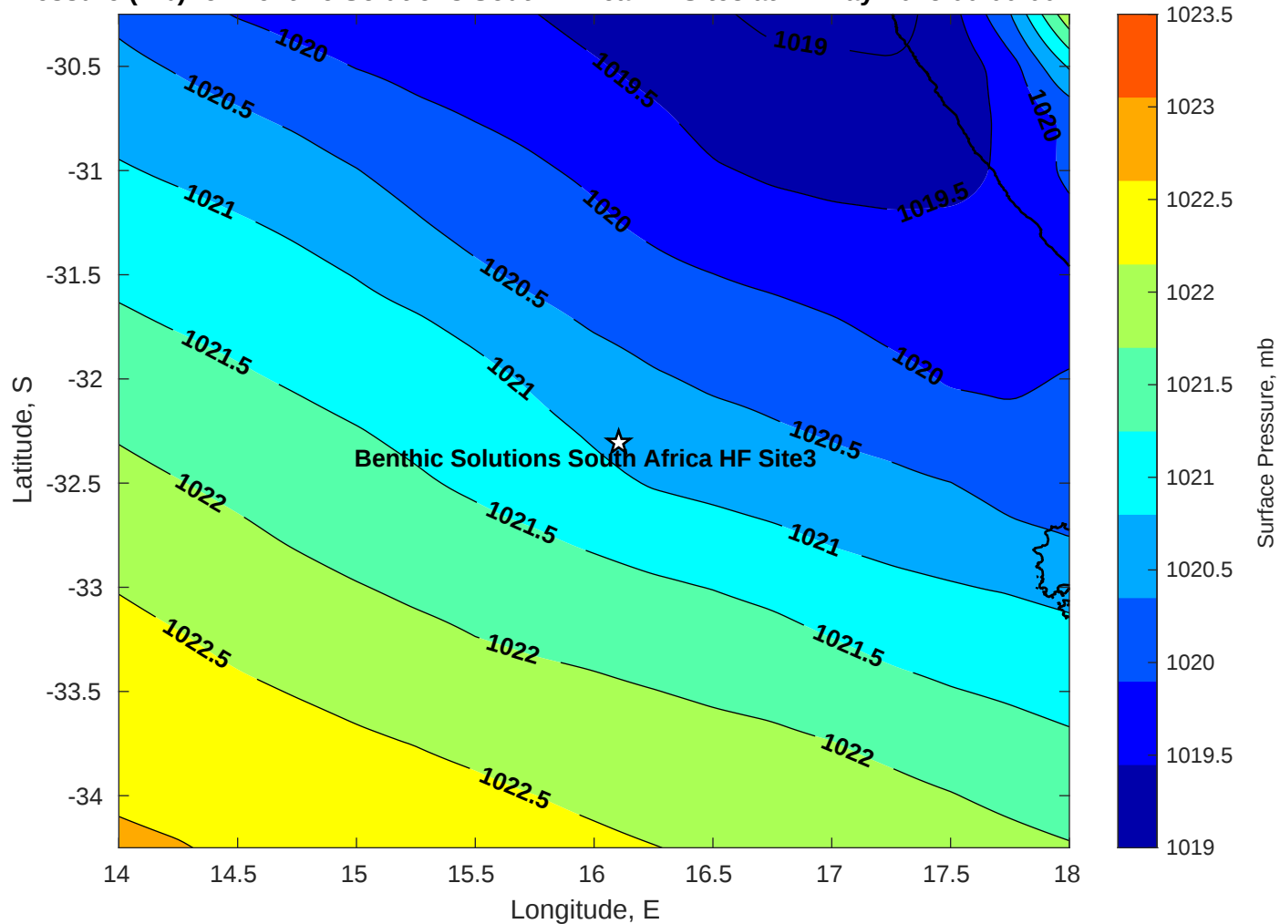
Surface Pressure (mb) for Benthic Solutions South Africa HF Site3 at 14-May-2025 00:00:00
